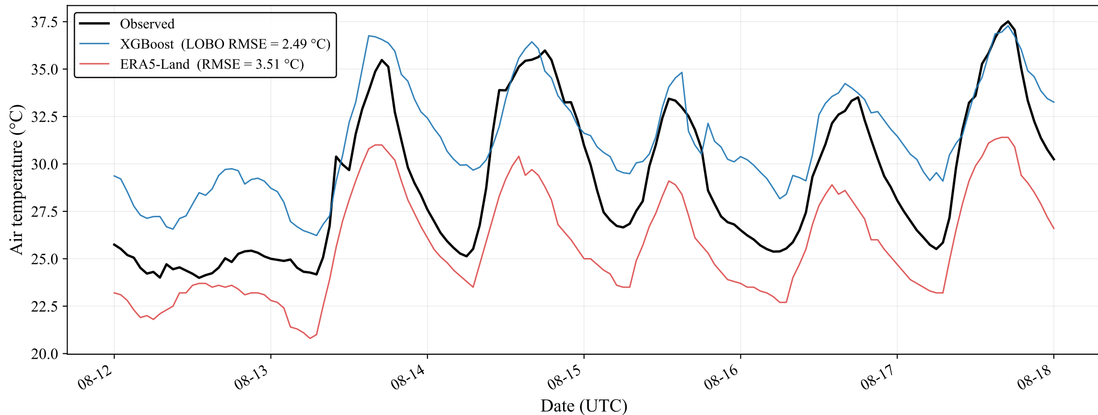
(a) Best fold (M04): XGBoost vs observed vs ERA5-Land (LOBO gain = +29.1%)
