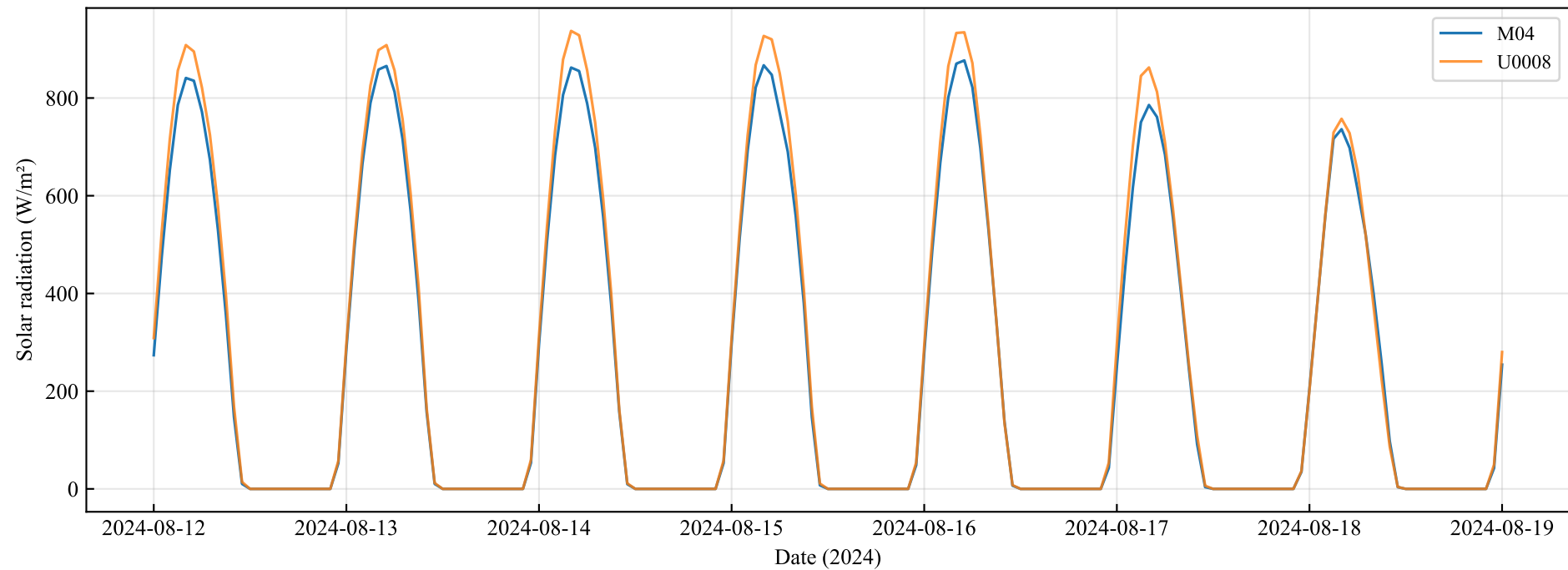
Fig.12a Hourly solar radiation at representative bridges (Aug 12-18, 2024)
