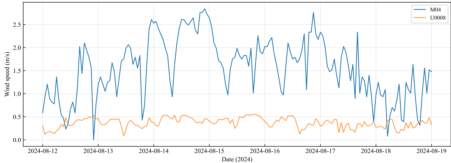
Fig.13a Hourly corrected wind speed at representative bridges (Aug 12-18, 2024)
