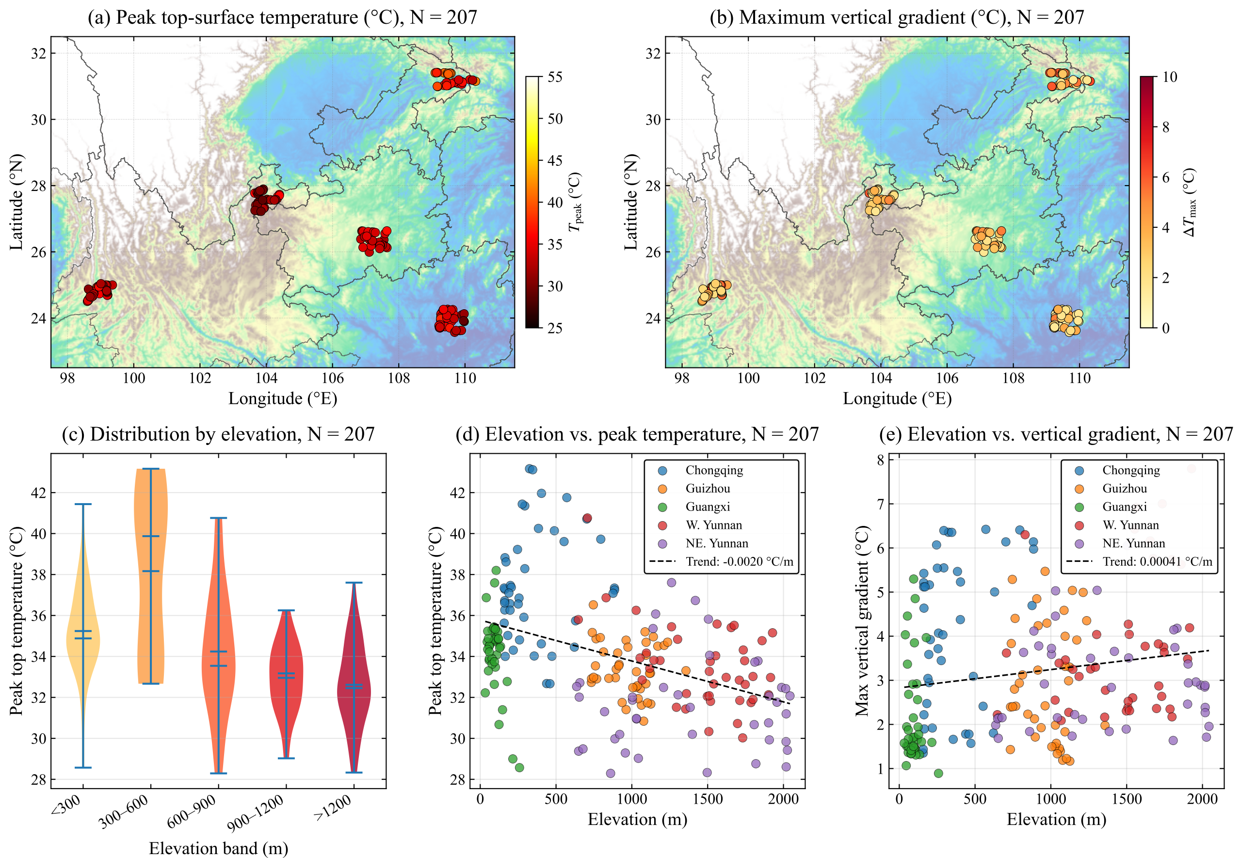
Figure 21 Cluster-scale temperature indicators for 207 concrete box-girder bridges (FEM driven by downscaled ERA5-Land boundary conditions, actual typical cross-sections).
