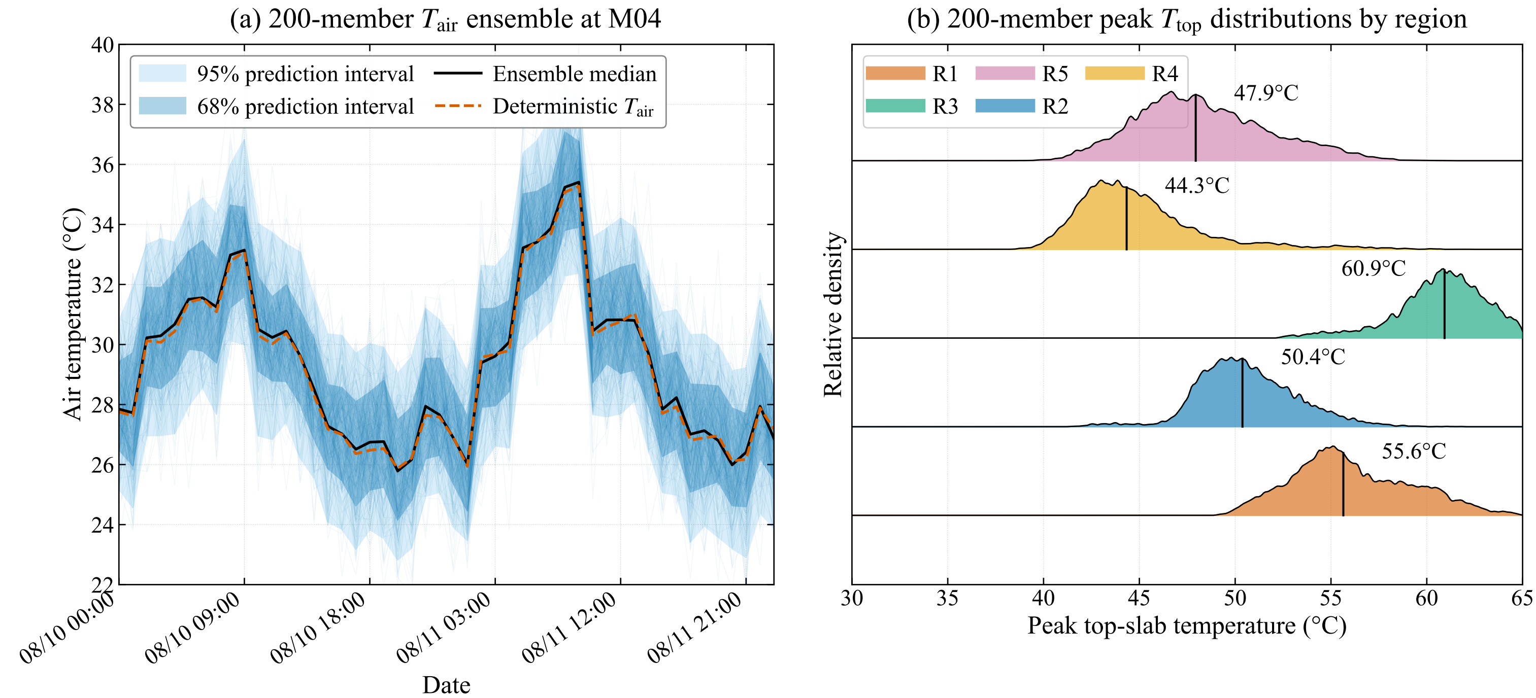
Figure 22 200-member Monte Carlo two-scale uncertainty propagation: (a) 200-member air-temperature ensemble cloud at M04 with 68% and 95% prediction intervals; (b) ridge-density distributions of 200-member peak top-slab temperatures for 207 bridges grouped by five regions.
