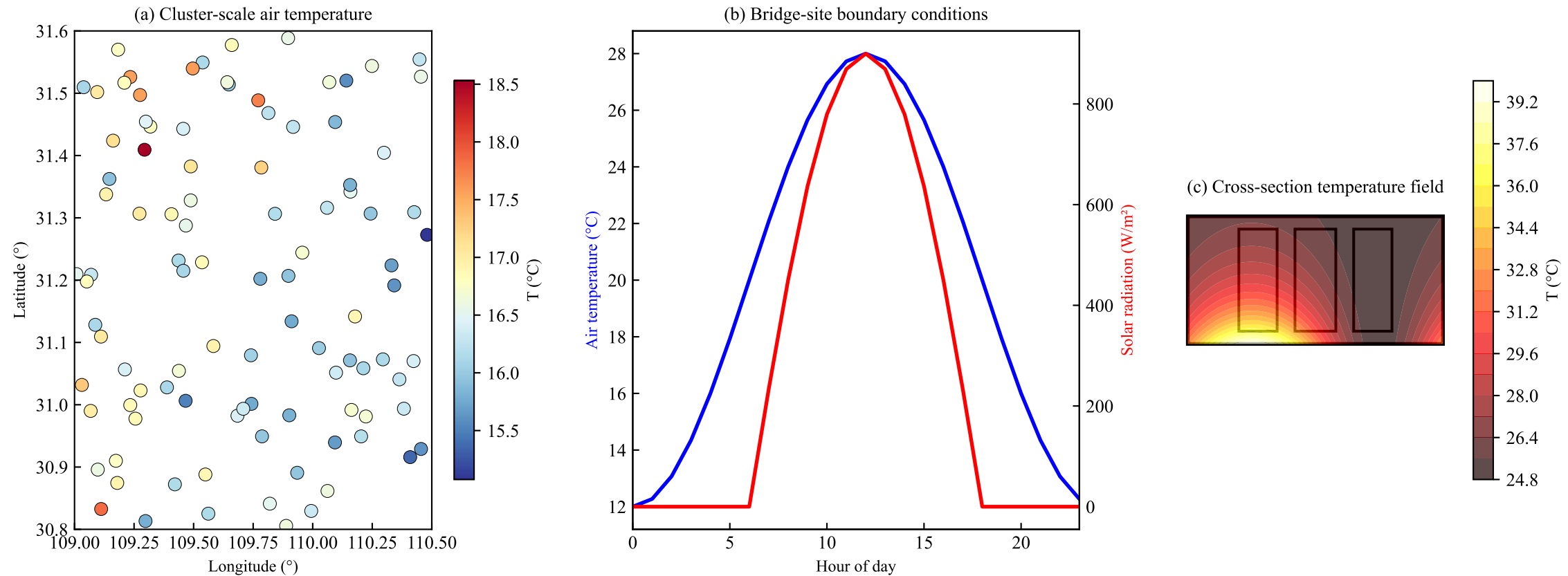
Fig.19 Multi-scale synthesis from satellite/reanalysis data to bridge-section temperature field
