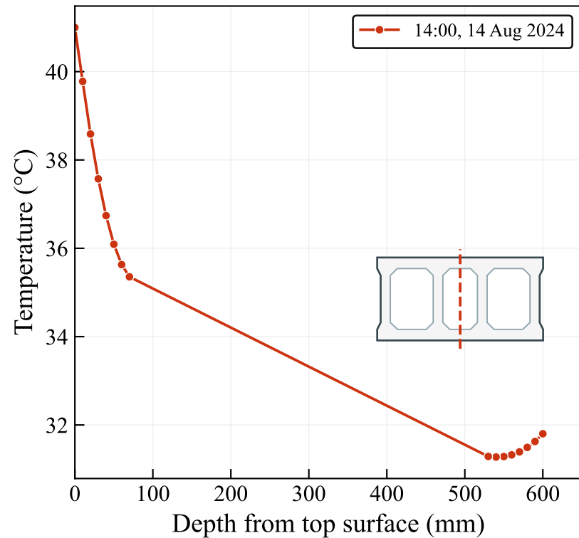
Fig. 17 Vertical temperature gradients at 14:00 on 14 August 2024
