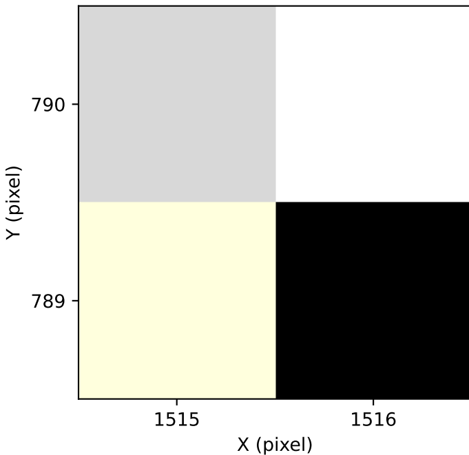
(a) H \alpha wing mean 6560.800–6561.250 Å
