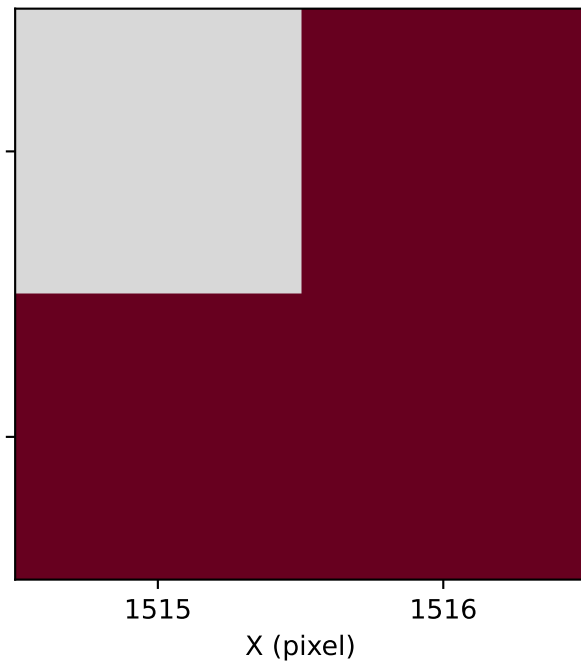
(c) Upper cloud: v_U
