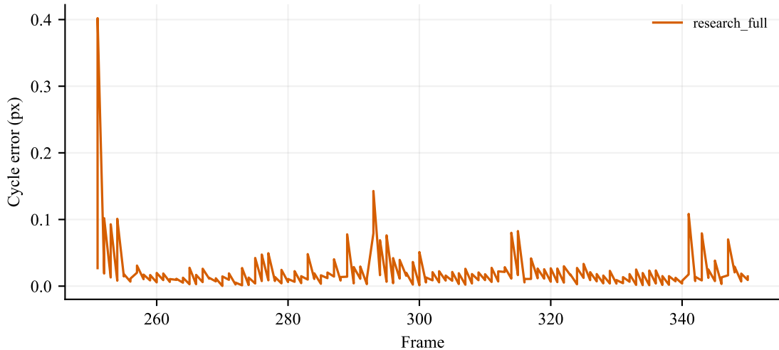
Four-view cycle consistency
