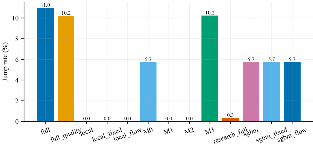
Jump rate (%)
