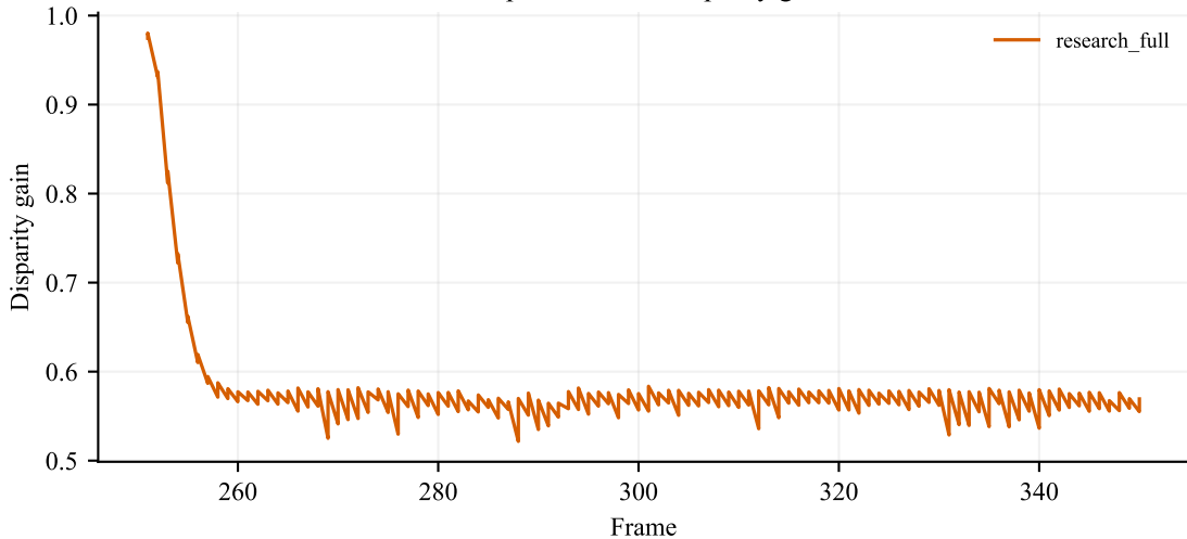
Adaptive Kalman disparity gain
