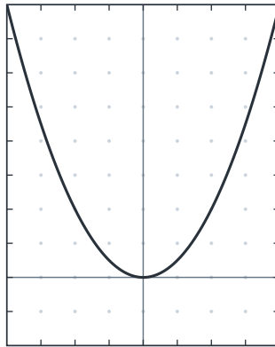
Figure 1: A quadratic function
