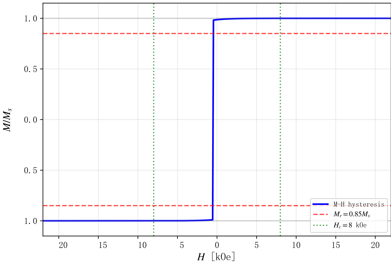
Hysteresis Loop of Ferromagnetic Material
