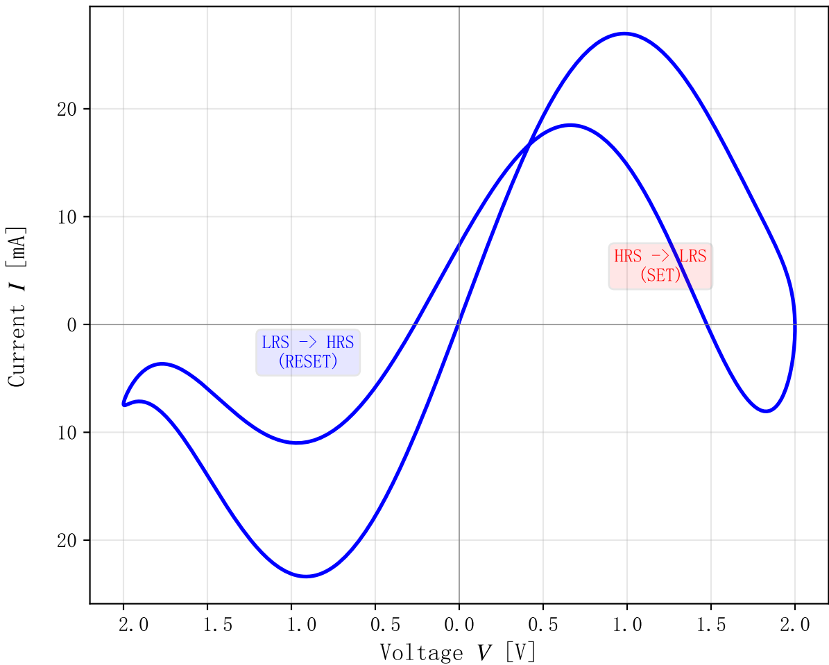
ReRAM Memristor: Pinched Hysteresis I-V
