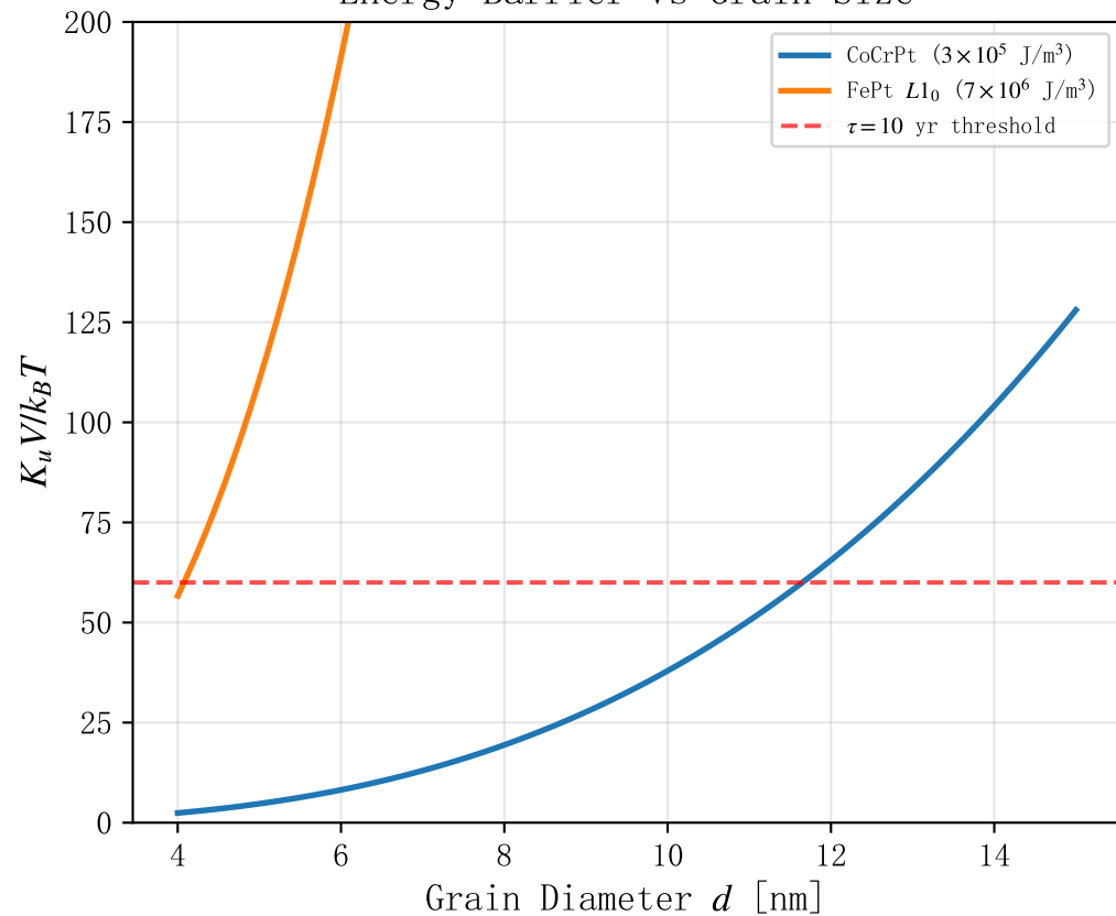
Energy Barrier vs Grain Size
