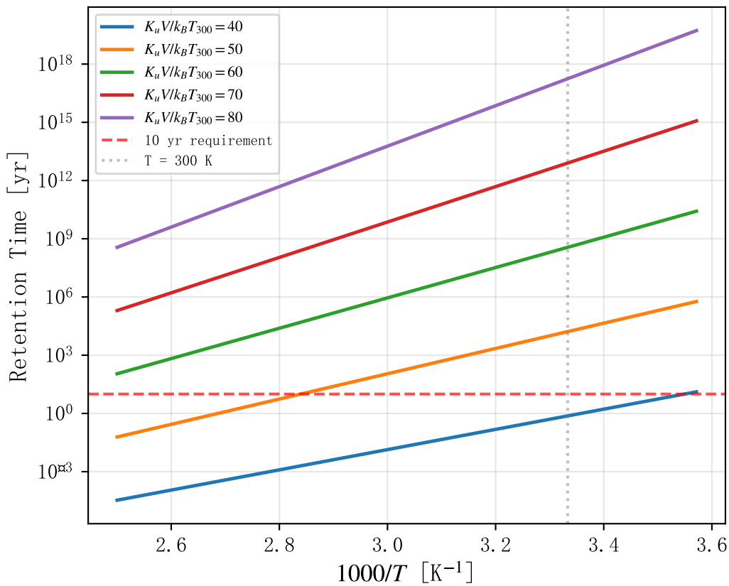
Arrhenius: \tau = \tau_0 \exp(K_u V / k_B T)
