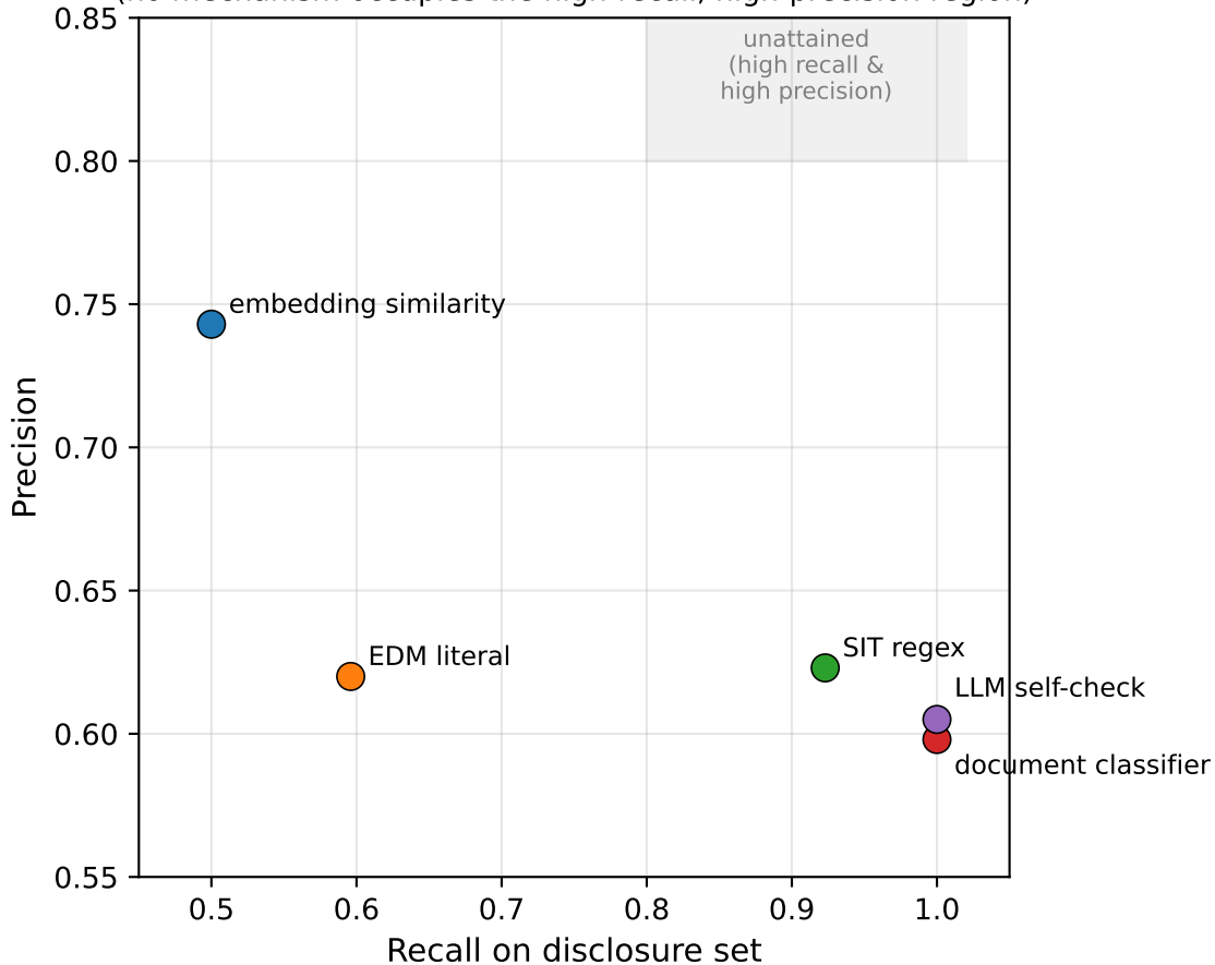
Output-layer detectors: recall-precision trade-off (no mechanism occupies the high-recall, high-precision region)
