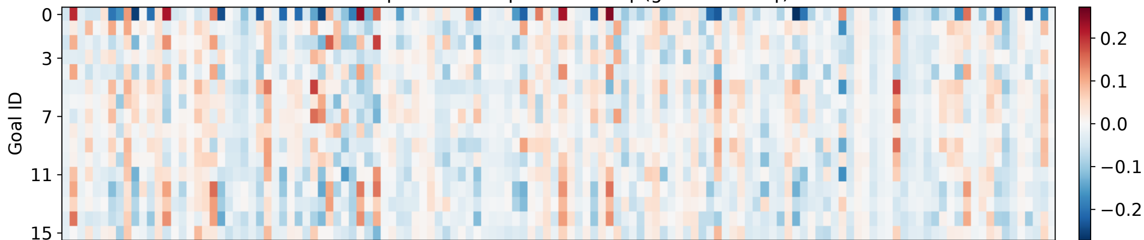
DGP_C15_HIT_JOINT_FILM_S99 75.04M frames · 16 goals × 128 hidden units · weights only Goal-specific scale parameter \Delta\gamma (gain = 1 + \Delta\gamma )
