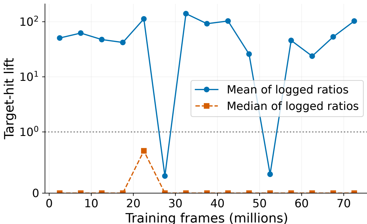
c Exploration
