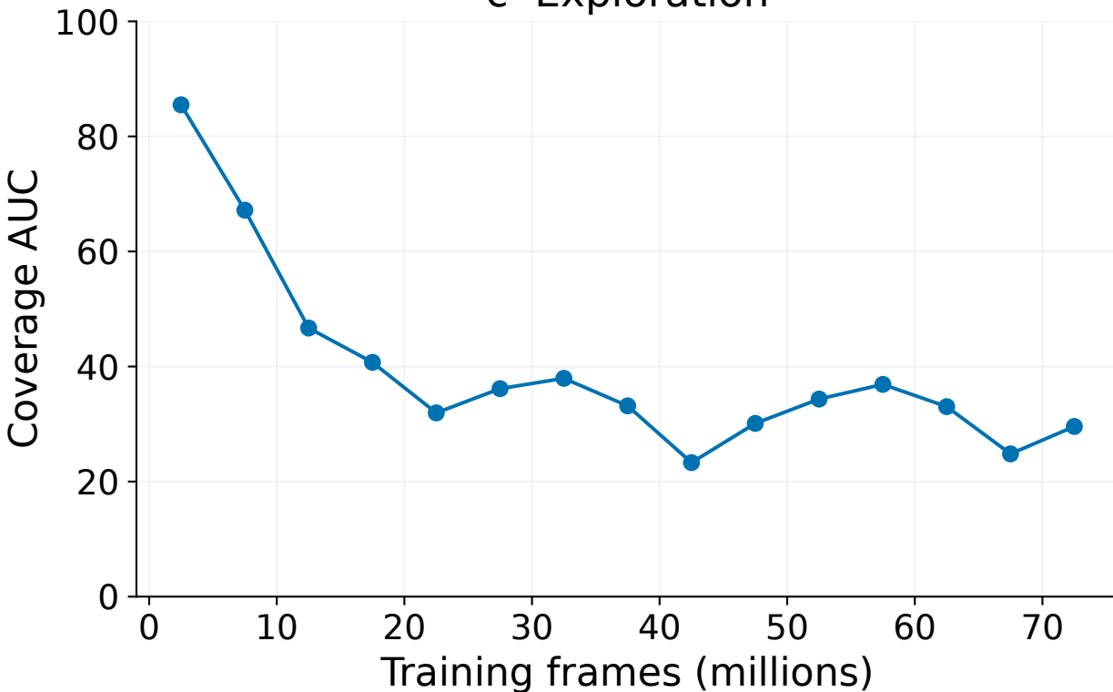
c Exploration
