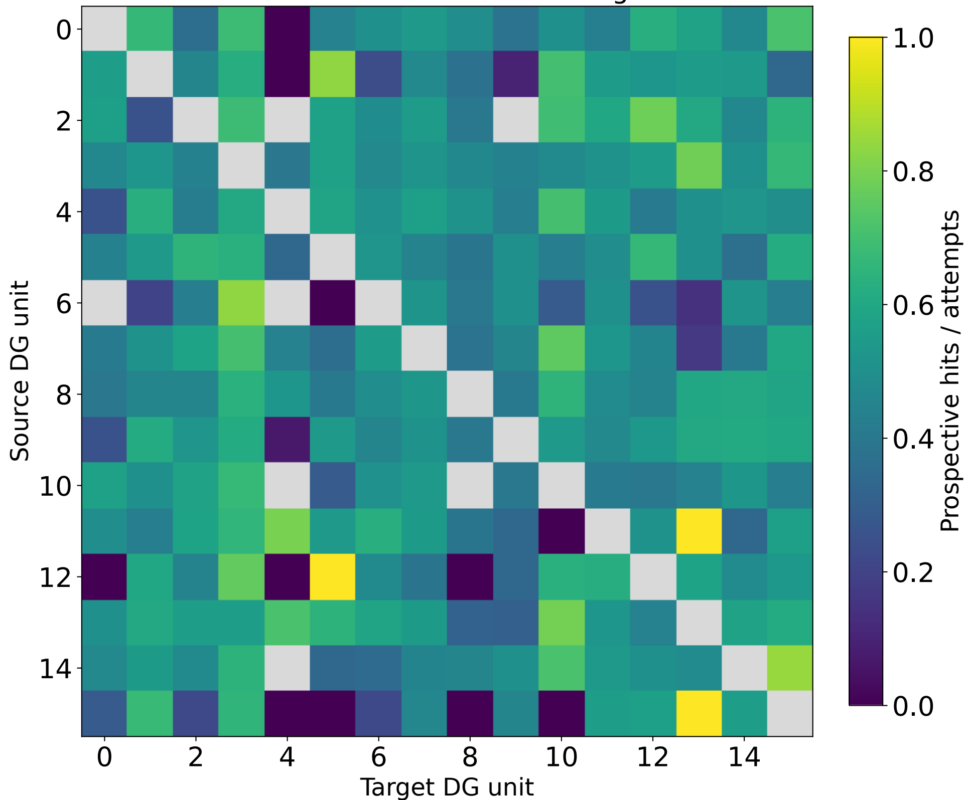
C15 seed 99 · None Stop 100M · 97 reliable stored edges
