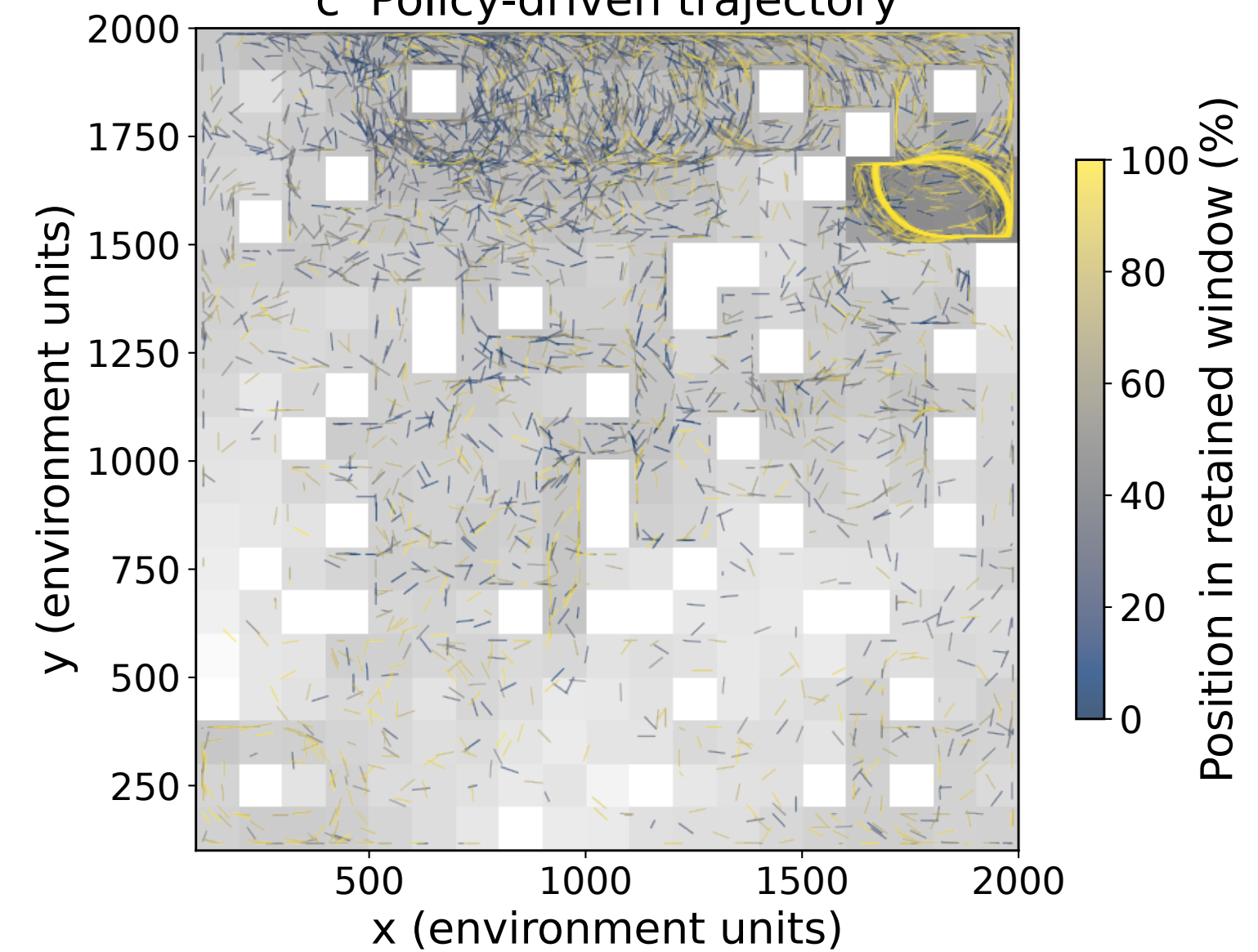
c Policy-driven trajectory
