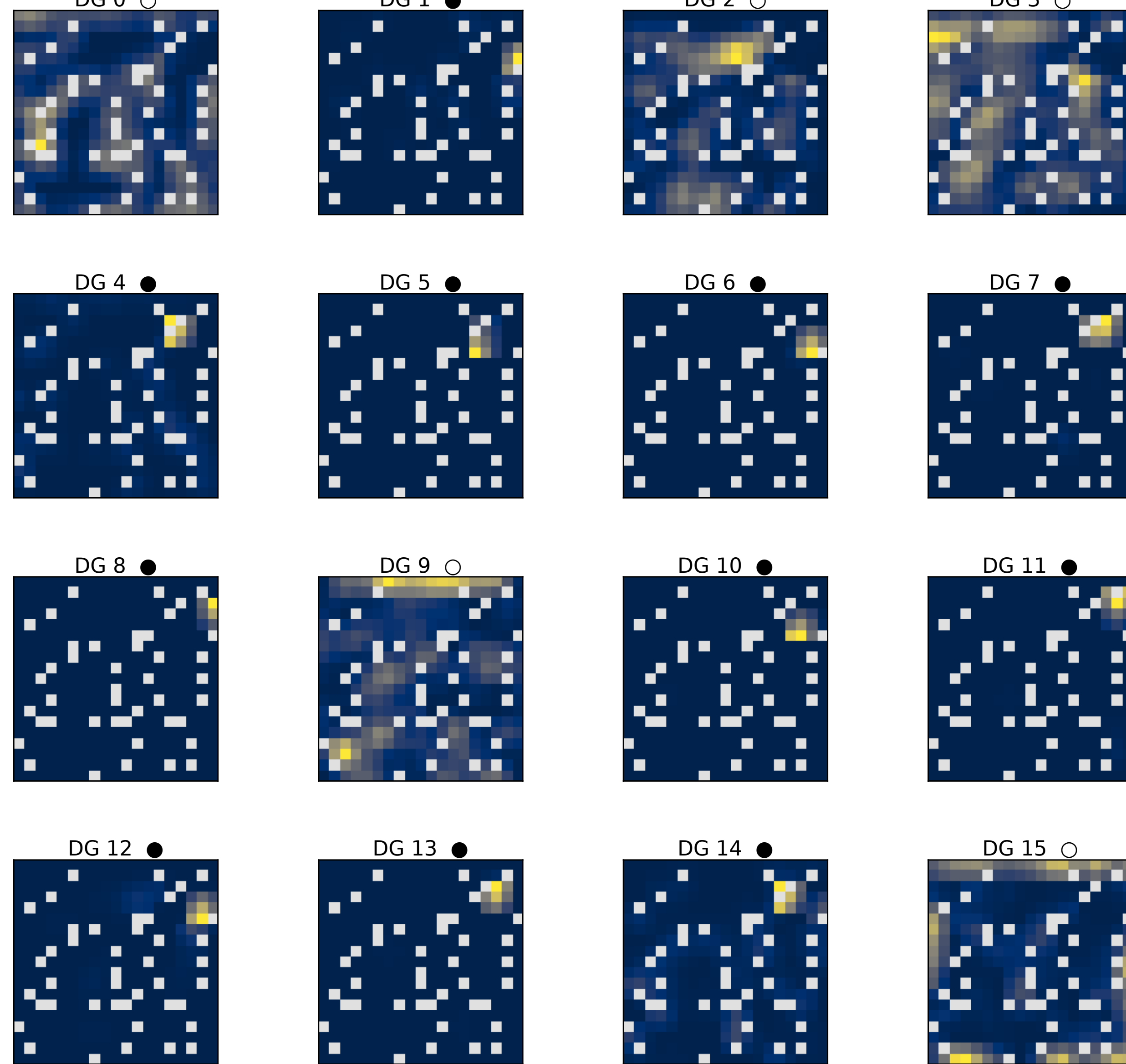
a Place fields
