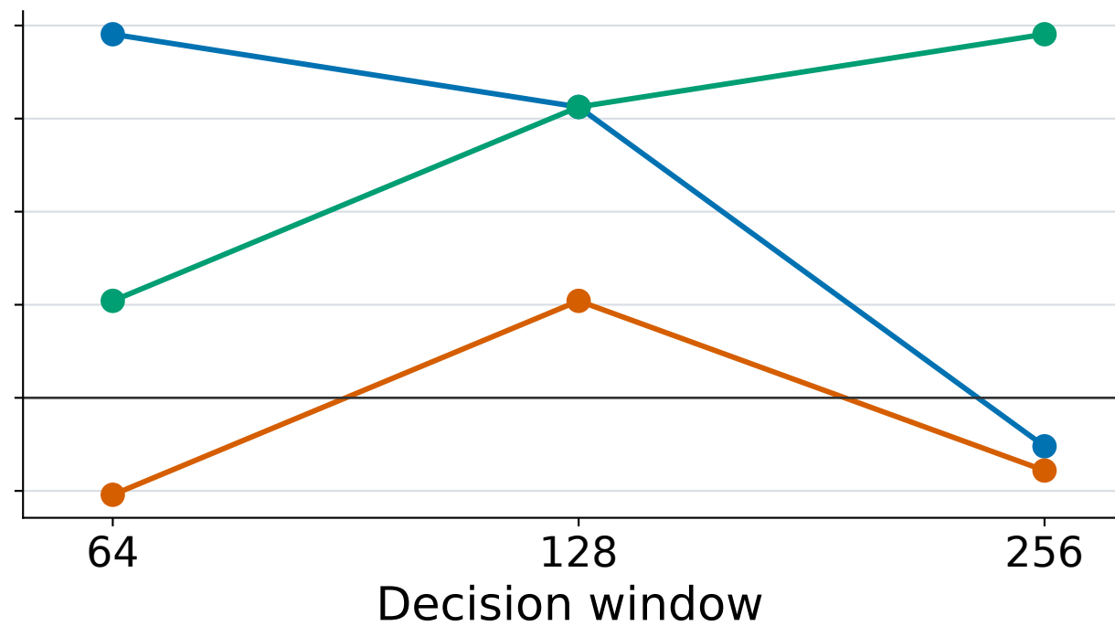
Learned-4 detector
