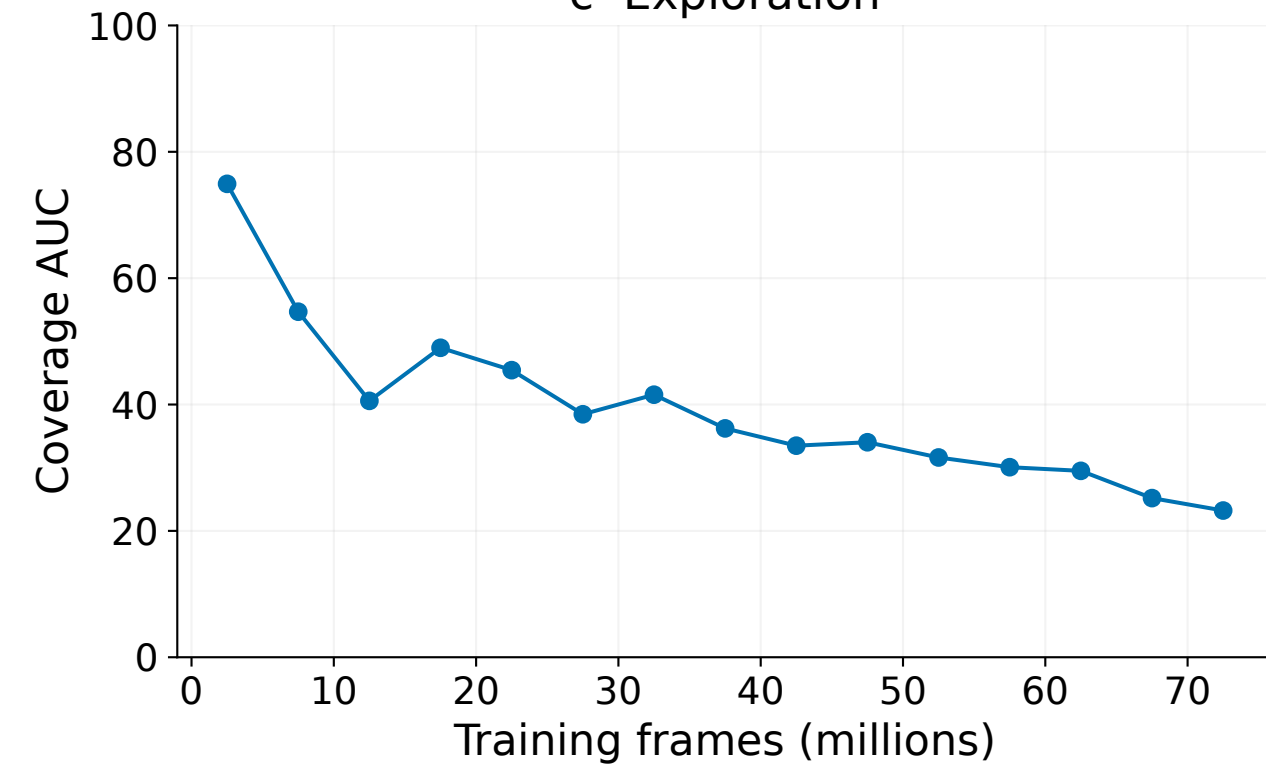
c Exploration
