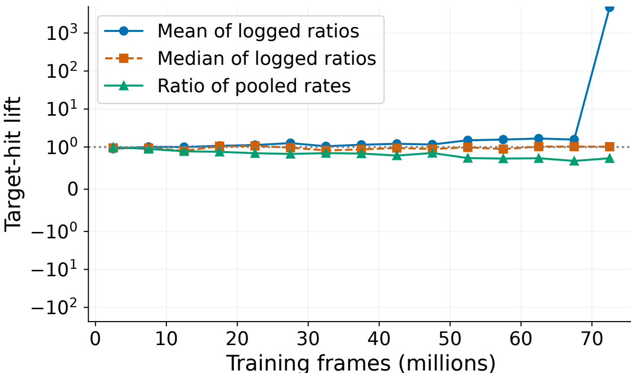
c Exploration
