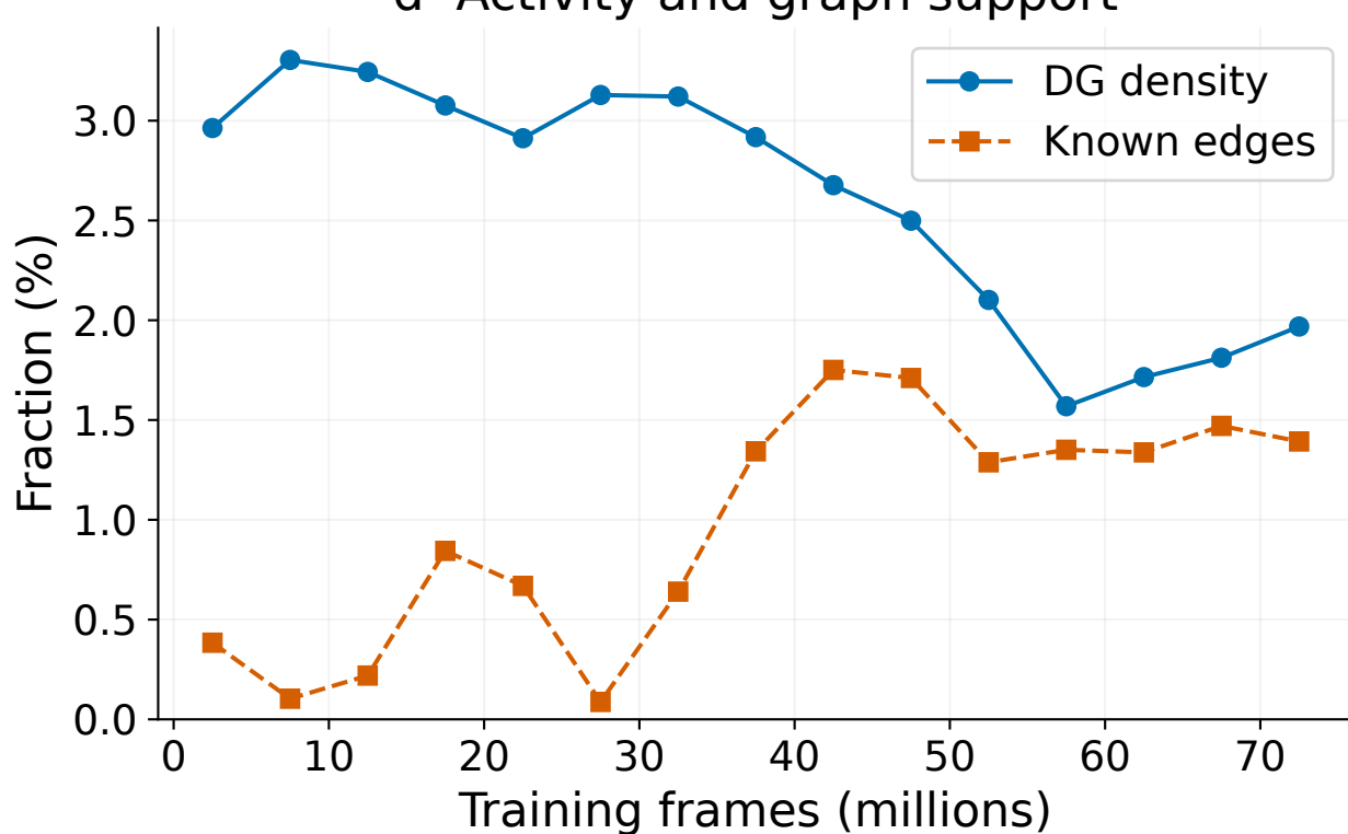
d Activity and graph support
