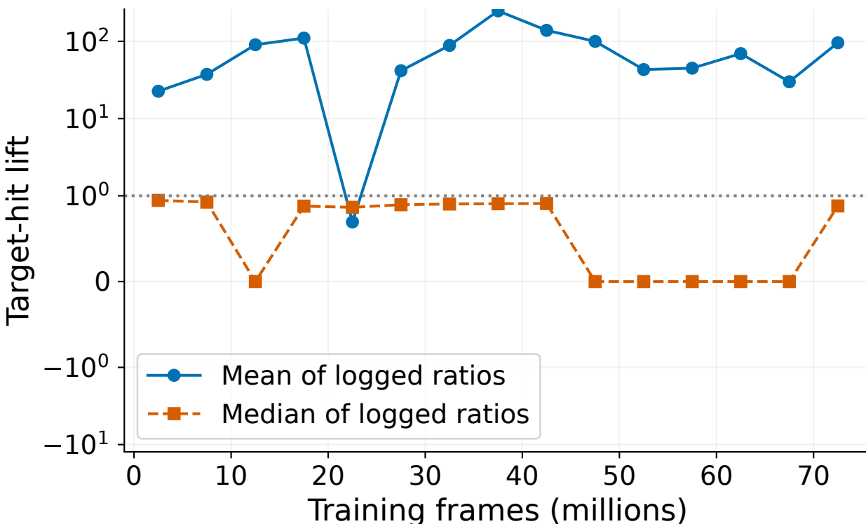
c Exploration
