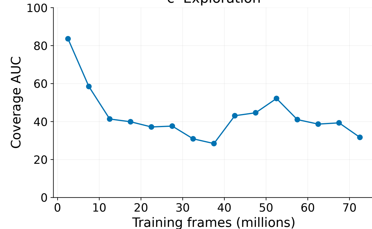
c Exploration
