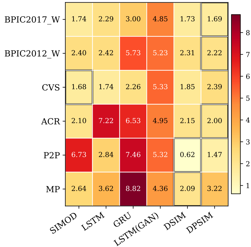
Temporal Perspective CED
