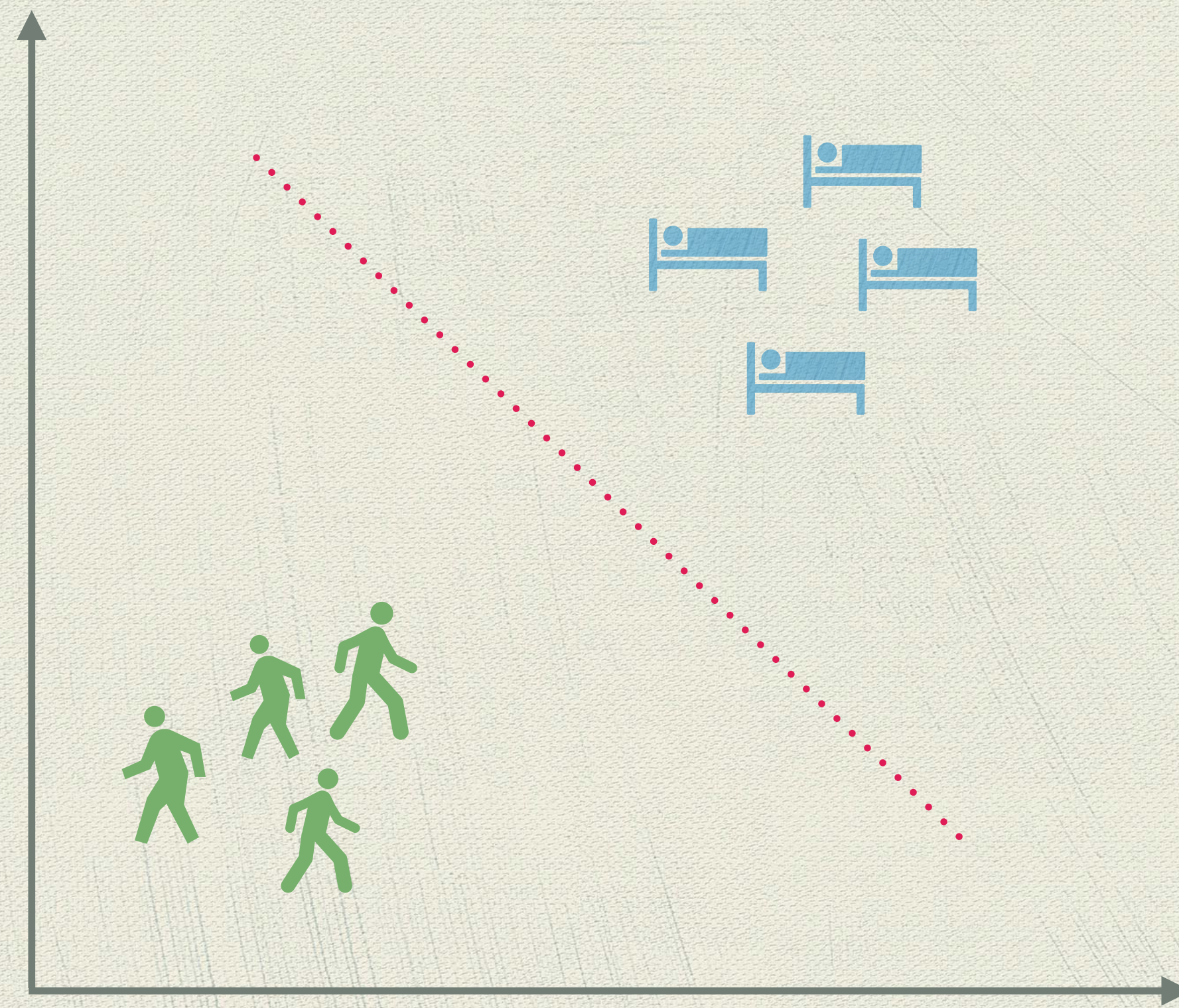
Expectation: clusters
