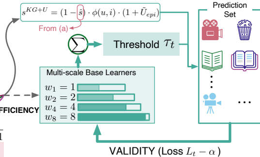
(c) SA-OKAC: Validity-Efficiency Separation
