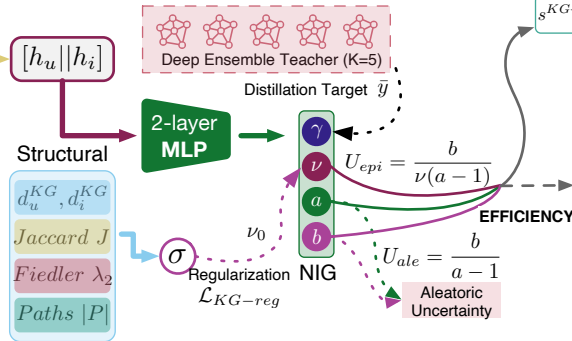
(b) KGUP: Topology as Epistemic Evidence
