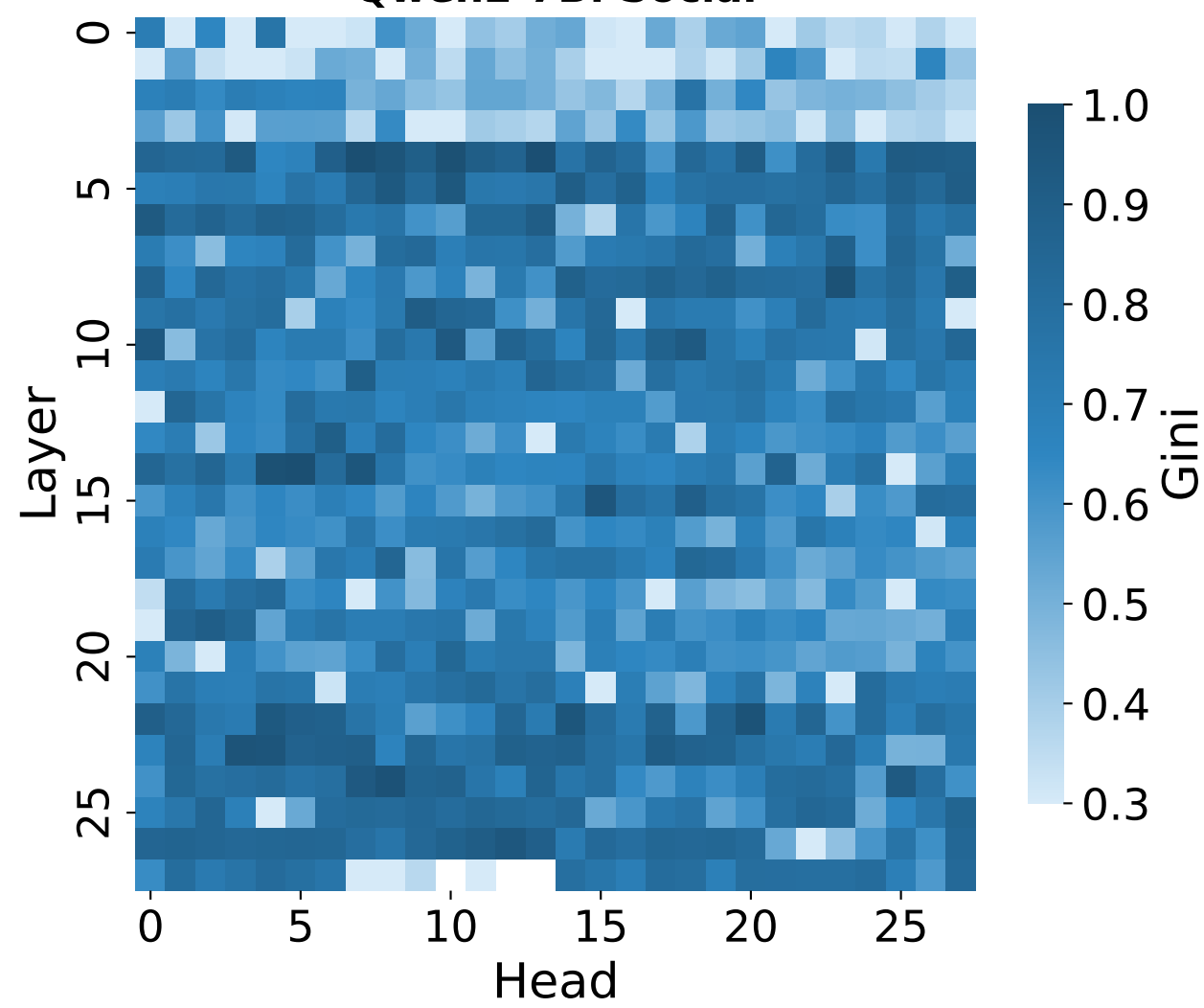
Qwen2-7B: Social
