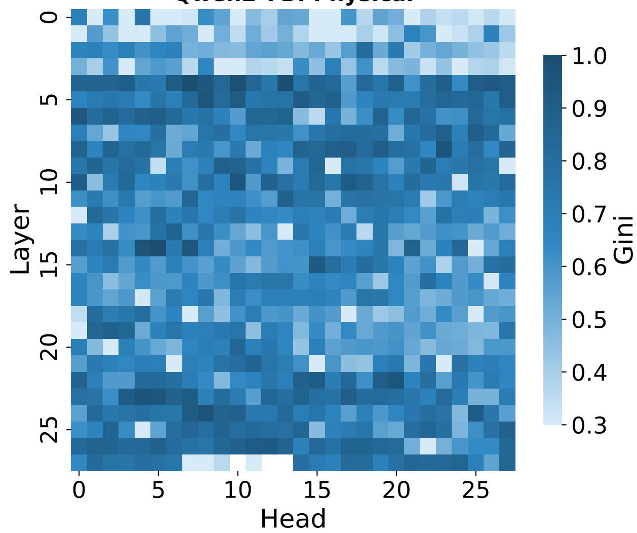
Qwen2-7B: Physical
