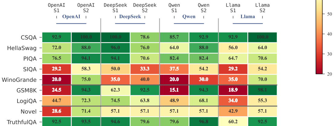
(b) Per-Source Accuracy Across Model Families
