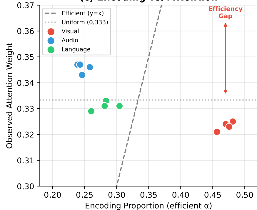
(c) Encoding vs. Attention
