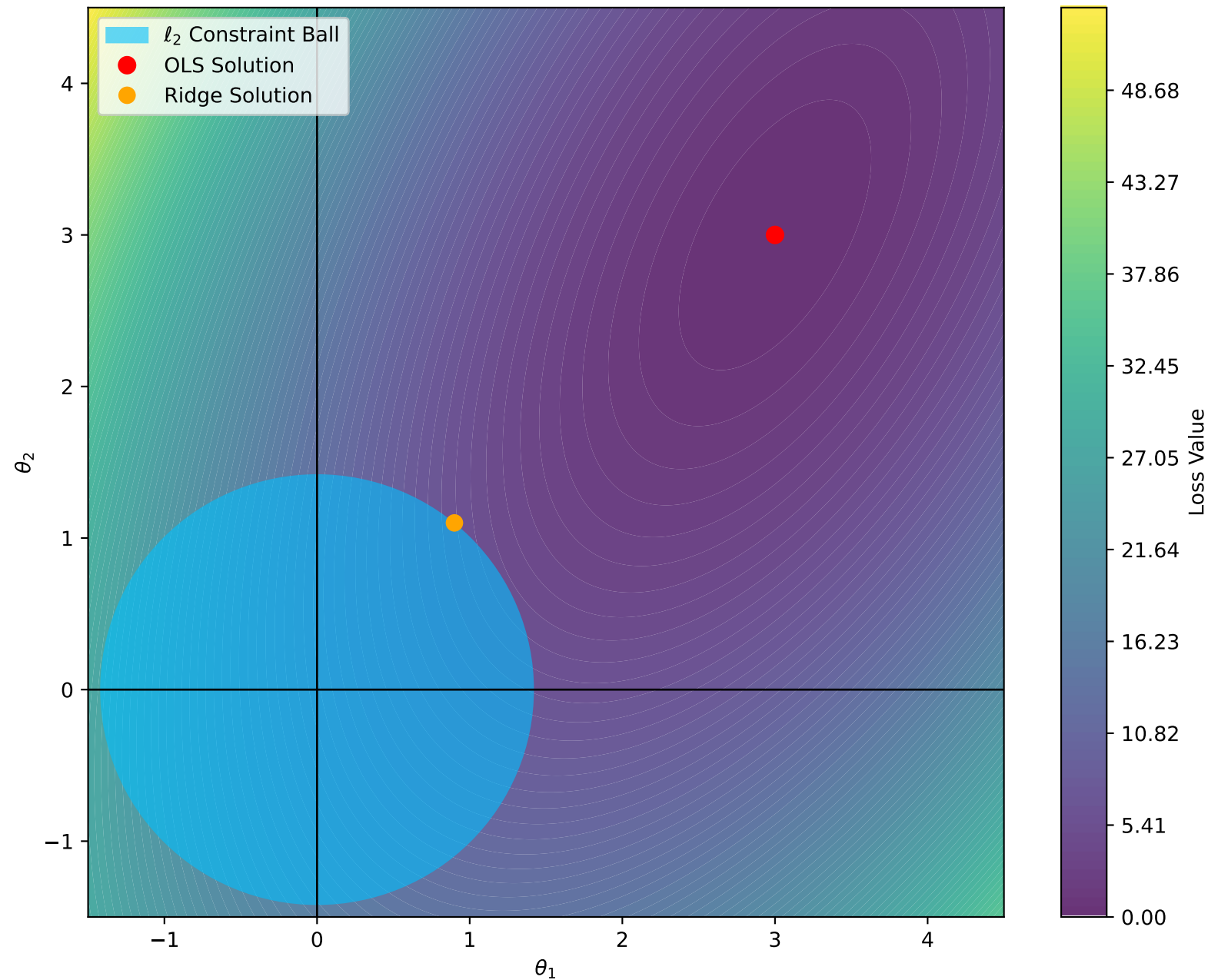
Geometric Interpretation of Ridge Regression ( \ell_2 ball)
