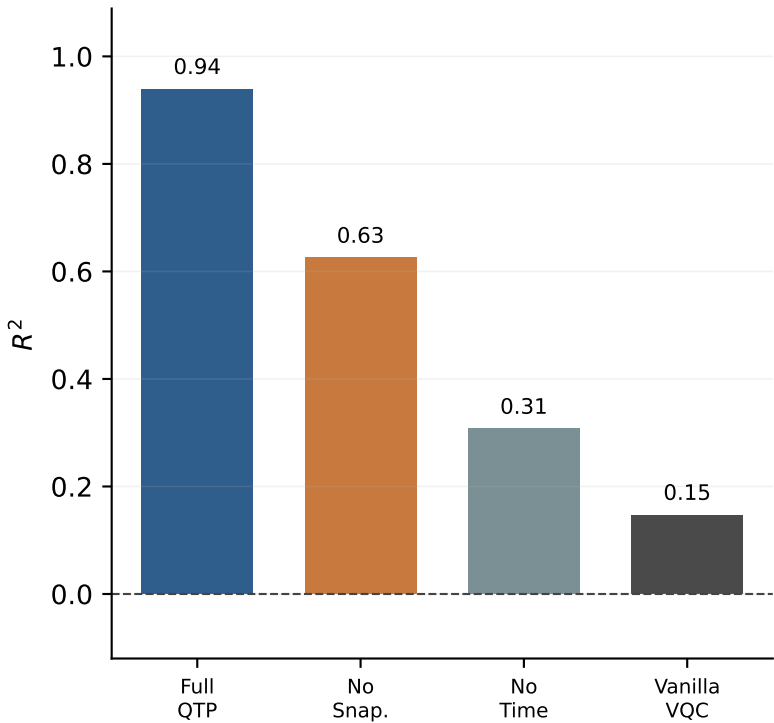
Toy 2 performance
