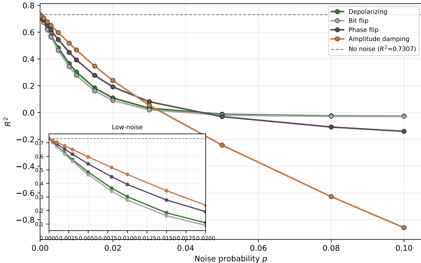
Gate noise + finite-shot robustness - lorenz (reloaded)
