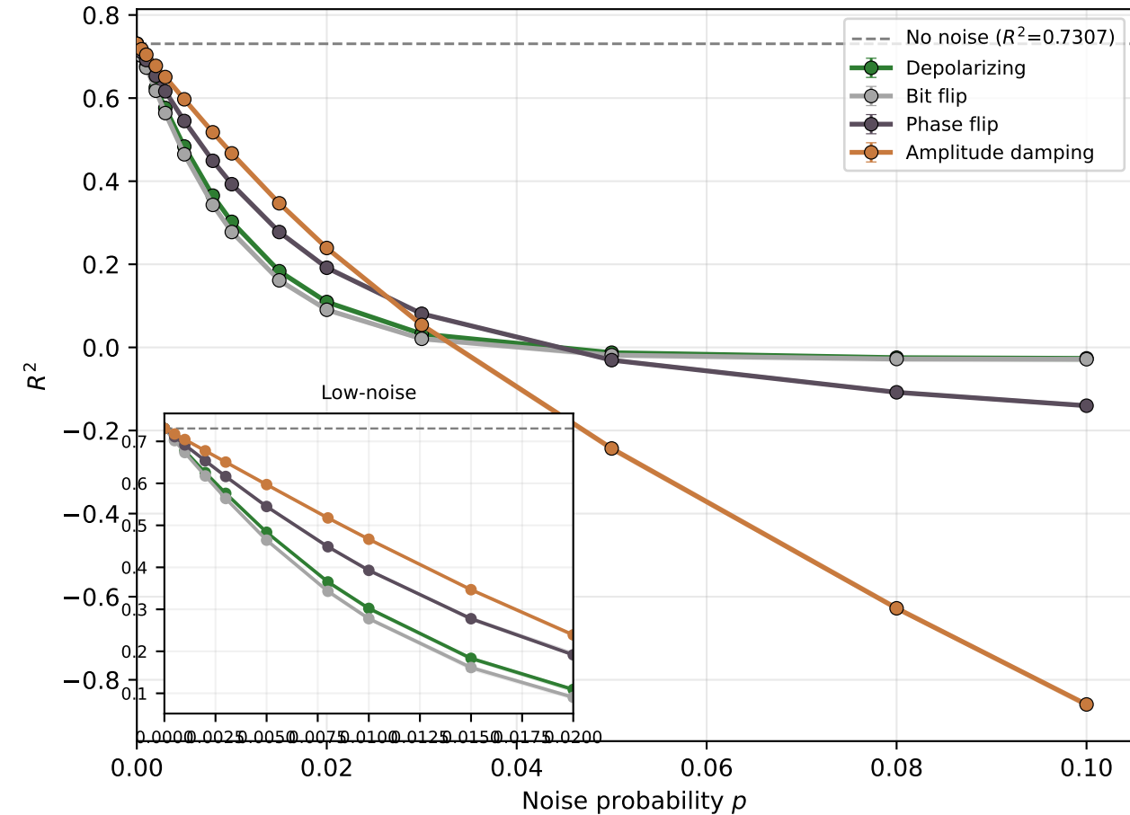
Gate noise + finite-shot robustness - lorenz
