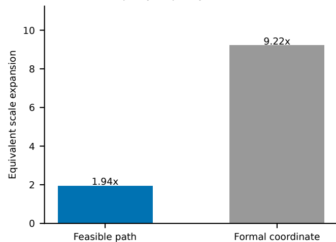
d Soft proxy: capacity at lambda Q = 1
