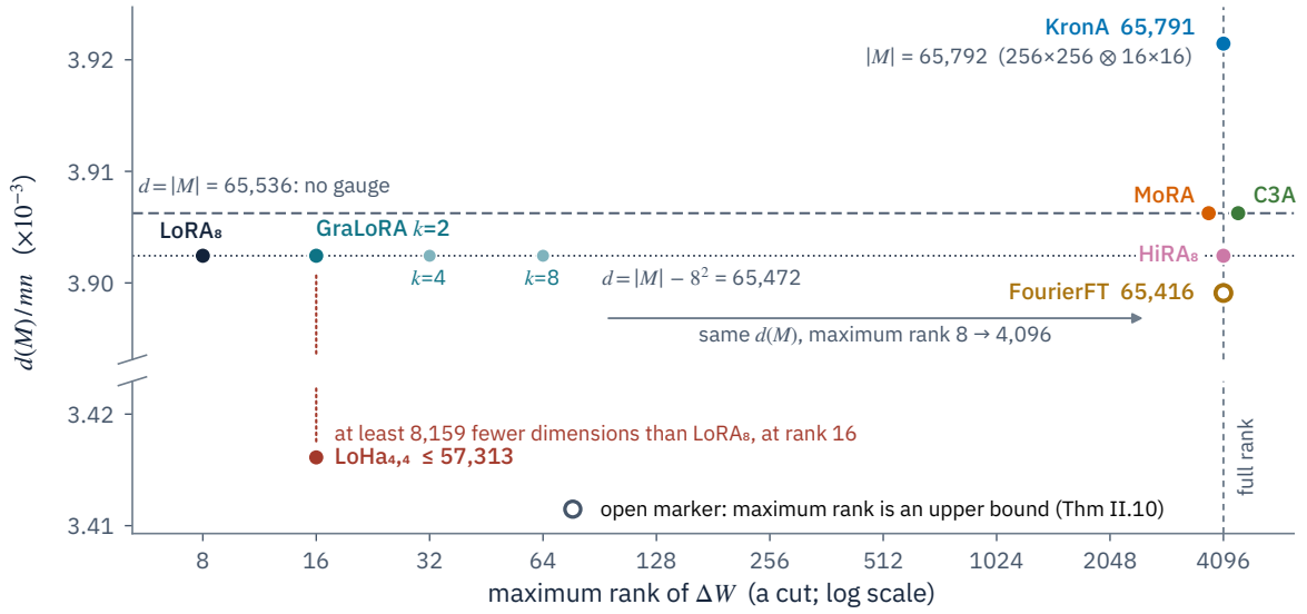
Figure 4. Rank is not volume (Theorem II.10, Proposition II.12). One 4096 \times 4096 layer at the budget of LoRA 8 (Hu et al., 2021), |M| = 8(m + n) = 65,536 . Each method is placed by the largest rank of \Delta W it can reach (horizontal, logarithmic scale), which is bounded by the narrowest cut of its diagram (Theorem II.10), and by its expressive dimension as a fraction of the layer, d(M)/(mn) (vertical, in units of 10^{-3} , with the axis broken between 3.41 and 3.90), from the gauge census of Proposition II.12. The dashed line is d = |M| , a method without gauge, and the dotted line is d = |M| - 8^2 = 65,472 , the dimension of LoRA 8 with its GL 8 gauge. Along the dotted line the maximum rank runs from 8 for LoRA 8 , through GraLoRA (Jung et al., 2025) with k = 2, 4 and 8 blocks (the last two light), to full rank for HiRA 8 (Huang et al., 2025b). MoRA (Jiang et al., 2024) and C3A (Chen et al., 2024a) have no gauge and reach full rank; their points coincide and are drawn on either side of the full-rank line. FourierFT (Gao et al., 2024) loses one dimension for each sampled conjugate pair, and its maximum rank is known only through a bound (open marker). KronA (Edalati et al., 2022) is shown at the factor shapes closest to the budget. LoHa 4,4 (Hyeon-Woo et al., 2021), below the break, sits at the proved upper bound of its dimension: it reaches rank 16 with at least 8,159 fewer dimensions than LoRA 8 (Proposition II.12(c)). The parameters behind each point are in §E.6.
