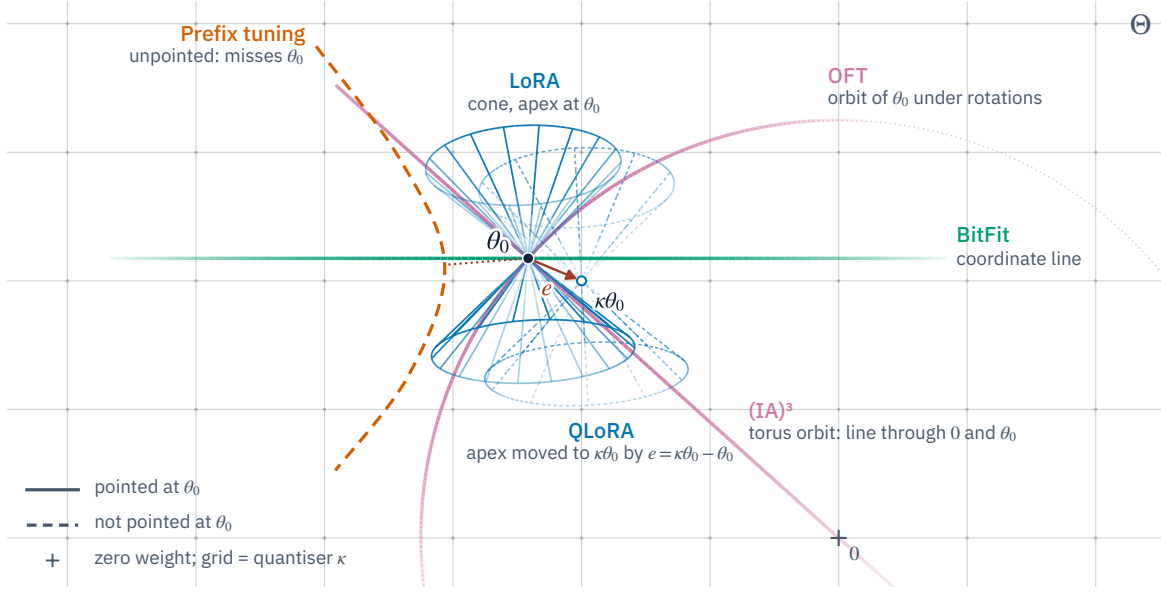
Figure 1. Fine-tuning moves a point. Weight space \Theta is drawn as a chart around the pretrained point \theta_0 ; the grid is the lattice of a round-to-nearest quantiser \kappa through the zero weight 0 (marked + ). Solid curves are image germs of methods pointed at \theta_0 (Definition I.2), drawn darkest near \theta_0 because only the germ there matters. LoRA (Hu et al., 2021) is the cone \theta_0 + \mathcal{M}_{\leq r} with its apex at \theta_0 (Theorem II.2), shown as the rank- \leq 1 double cone x^2 = y^2 + z^2 of the symmetric 2 \times 2 slice in perspective. OFT (Qiu et al., 2023) is the orbit of \theta_0 under rotations, an arc of the circle about 0 through \theta_0 , the rest of which is dotted. (IA) 3 (Liu et al., 2022a) is a torus orbit, whose closure is the line through 0 and \theta_0 (Theorem II.5). BitFit (Ben-Zaken et al., 2021) moves along a coordinate line, parallel to the grid. The dashed curves are not pointed at \theta_0 . Prefix tuning (Li and Liang, 2021) extends the network and is unpointed (Definition VI.1); drawn in weight space it is a curve that misses \theta_0 , at the distance marked by the dotted segment. QLoRA (Dettmers et al., 2023) is LoRA pointed at the nearest grid node \kappa\theta_0 , so its cone is LoRA’s cone translated by the defect e = \kappa\theta_0 - \theta_0 (red arrow), and \theta_0 is off its image unless rank e \leq r (Proposition V.2).
