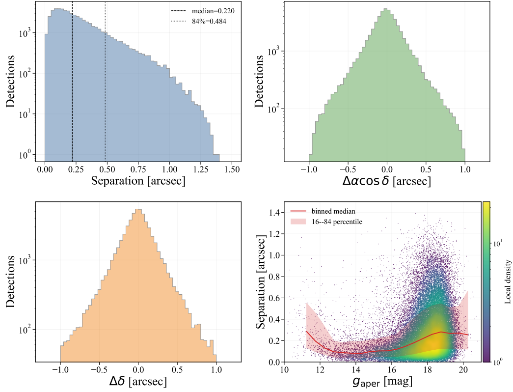
Fig. 7: Astrometric residual diagnostics. The panels show the observed-minus-predicted separation, \Delta\alpha\cos\delta , \Delta\delta , and separation as a function of the adopted aperture magnitude g_{\text{aper}} . In the lower-right panel, the solid curve and shaded region indicate the binned median and 16th–84th percentile range in magnitude bins.
