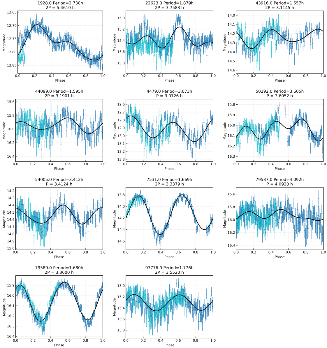
Fig. 11: Phase-folded light curves for the 11 high-confidence period measurements in the combined GOTTA Prototype and 60 cm Schmidt validation sample. Blue and cyan points denote the photometric measurements used in the folded light curves, gray points mark rejected or lower-weighted measurements, and black curves show the adopted Fourier models. Each panel gives the object identifier and the candidate period information used in the current period analysis.
