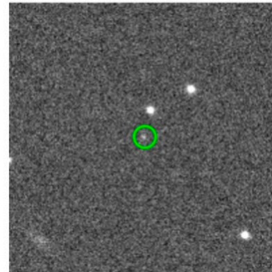
McKellar magnitude = 18.1915
