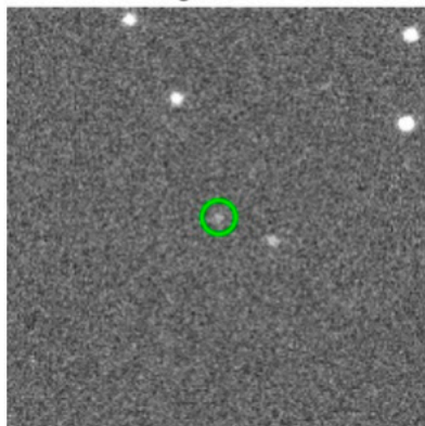
Silvain magnitude = 18.3375
