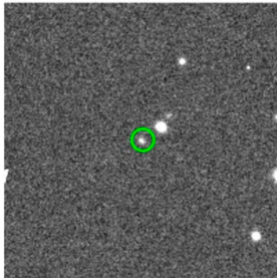
Barentine magnitude = 17.5078
