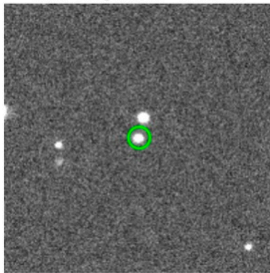
Arai magnitude = 16.0182
