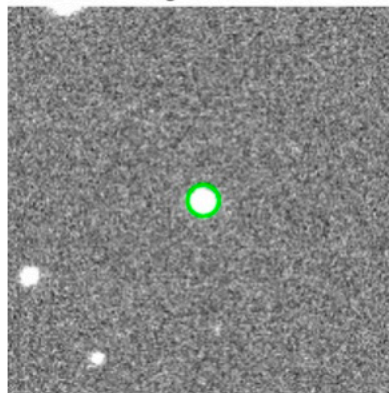
Nanon magnitude = 13.6306
