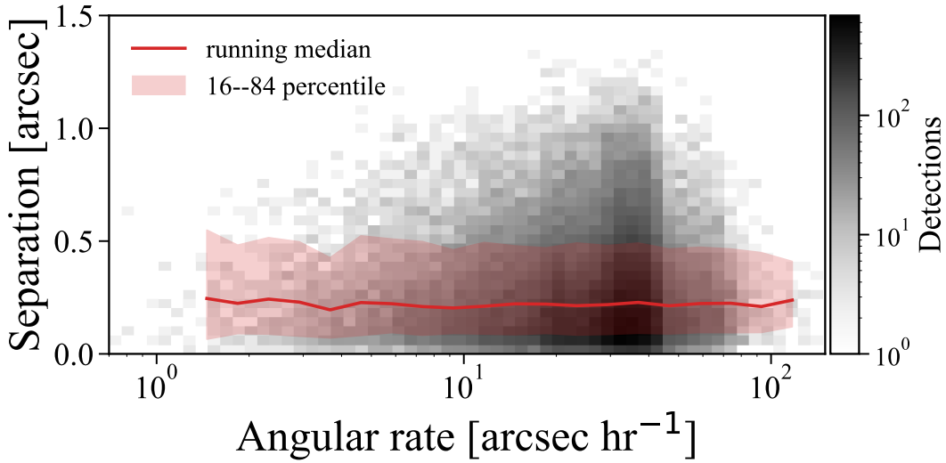
Fig. 6: Observed-minus-predicted separation as a function of sky-plane angular rate. The gray density map shows the dominant range of the recovered sample, while the red curve and shaded region show the running median and the 16th–84th percentile range in logarithmic rate bins. Most detections lie at moderate angular rates, where the residual distribution remains close to the full-sample behavior. A small number of higher-rate detections are excluded from the displayed range for clarity but are included in the binned statistics.
