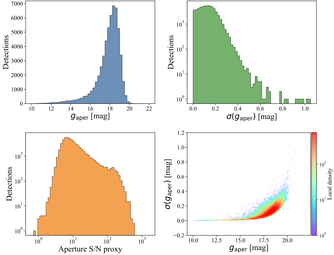
Fig. 4: Aperture-photometry diagnostics for recovered known asteroids. The adopted aperture follows the optimal aperture defined by the GOTTA basic photometric pipeline. The panels show the adopted aperture magnitude distribution, the corresponding magnitude-uncertainty distribution, the aperture S/N proxy, and the dependence of magnitude uncertainty on adopted aperture magnitude. The last panel is shown as a density map to emphasize the dominant distribution of faint asteroid detections.
