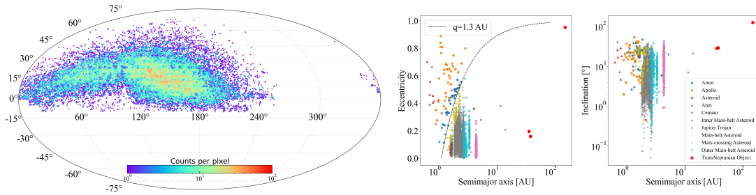
Fig. 3: Left: detection-level sky distribution of recovered known asteroids in equatorial coordinates, binned with HEALPix n_{\text{side}} 64 . The color scale is clipped at 100 detections per pixel for readability. Right: orbital-element distribution of the recovered known-object sample.
