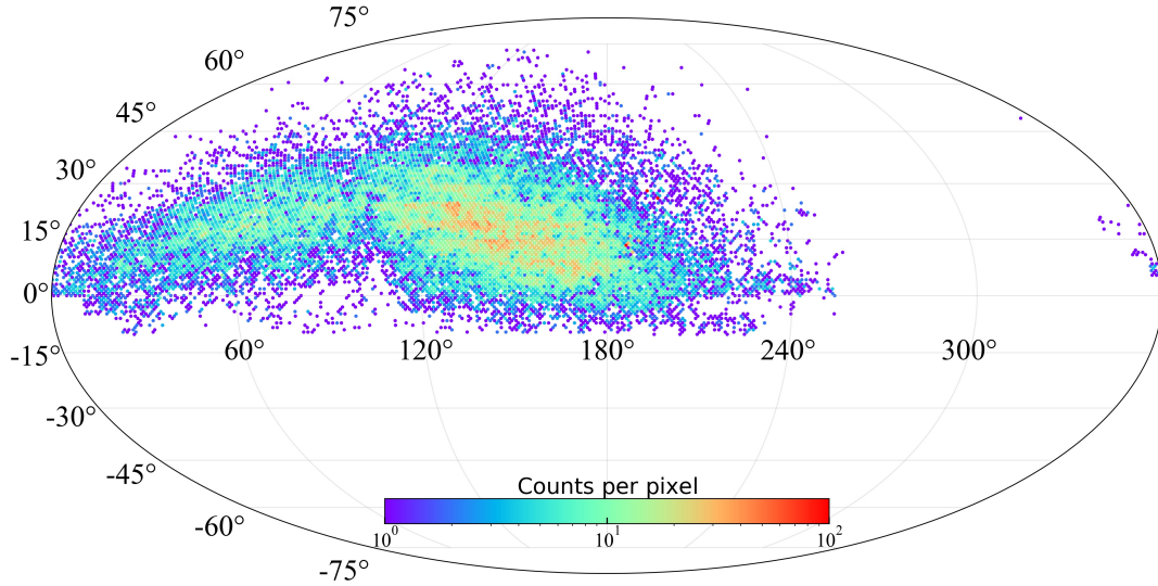
Fig. 3: Detection-level sky distribution of recovered known asteroids in equatorial coordinates, binned with HEALPix n_{\text{side}} 64 . The color scale is clipped at 100 detections per pixel for readability.
