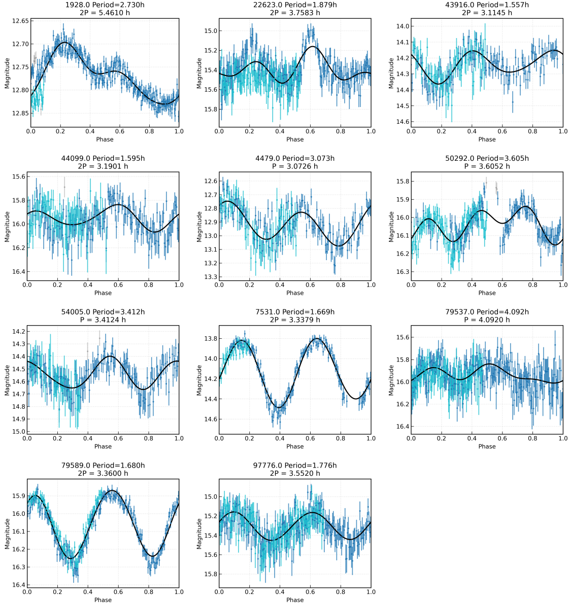
Fig. 11: Phase-folded light curves for selected high-quality period measurements in the combined GOTTA Prototype and 60 cm Schmidt validation sample. Blue and cyan points denote the photometric measurements used in the folded light curves, gray points mark rejected or lower-weighted measurements, and black curves show the adopted Fourier models. Each panel gives the object identifier and the candidate period information used in the current period analysis.
