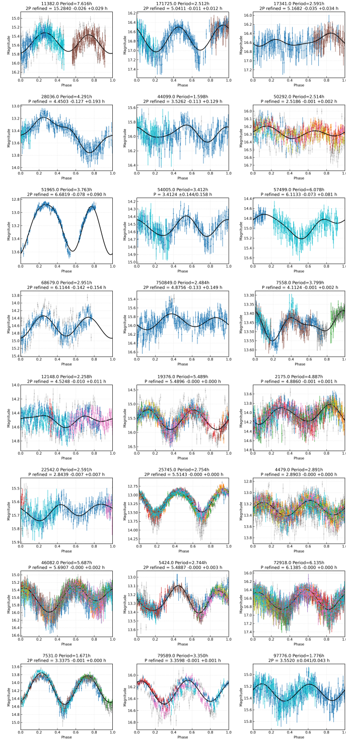
Fig. 11: Phase-folded light curves for the 24 objects in the updated combined GOTTA Prototype and 60 cm Schmidt validation sample. The two mosaics show the objects assigned reliable and questionable final quality flags, respectively. Colored points denote retained measurements from different data subsets, gray points mark rejected or lower-weighted measurements, and black curves show the adopted Fourier models. Each panel gives the object identifier and the candidate period information used in the current period analysis.
