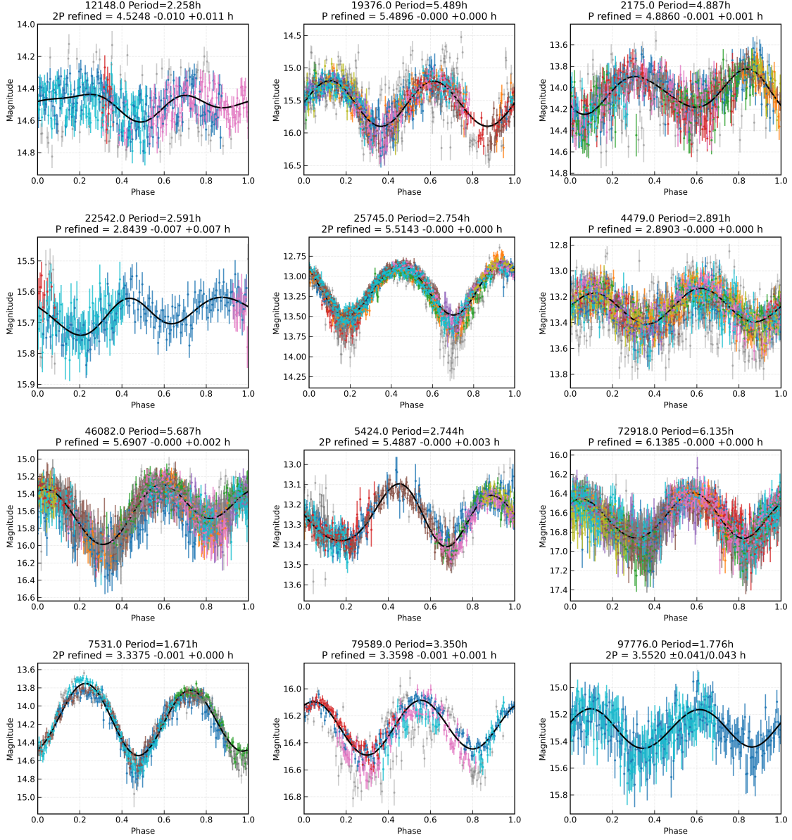
Fig. A.1: Phase-folded light curves for the 12 objects assigned reliable final quality flags in the updated combined GOTTA Prototype and Xinglong Schmidt validation sample. Colored points denote retained measurements from different data subsets, gray points mark rejected or lower-weighted measurements, and black curves show the adopted Fourier models. Each panel gives the object identifier and the candidate period information used in the current period analysis.
