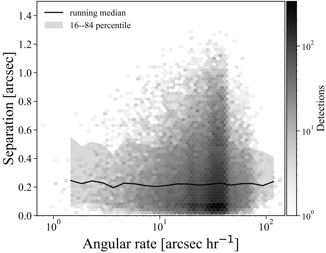
Fig. 6: Observed-minus-predicted separation as a function of sky-plane angular rate. The gray density map shows the dominant range of the recovered sample, while the black curve and shaded region show the running median and the 16th–84th percentile range in logarithmic rate bins. Most detections lie at moderate angular rates, where the residual distribution remains close to the full-sample behavior. A small number of higher-rate detections are excluded from the displayed range for clarity but are included in the binned statistics.
