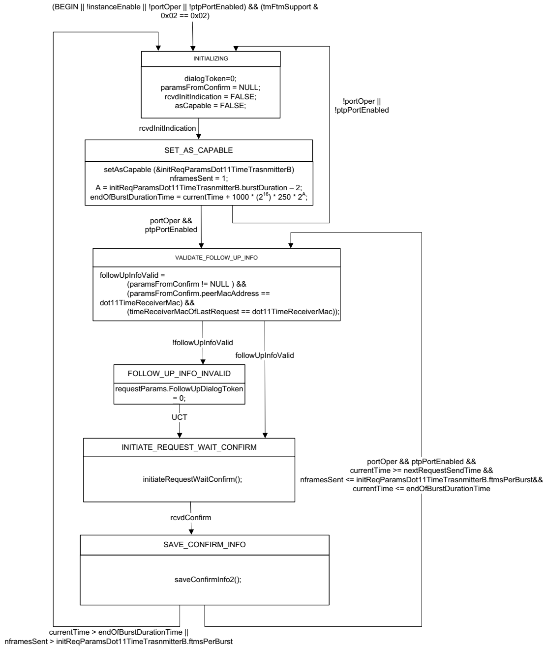
Figure 12-6—TimeTransmitter state machine B (a) For TM, not invoked and (b) For FTM, receives initial FTM request from timeReceiver and sends information received from upstream to timeReceiver in successive FTM frames
