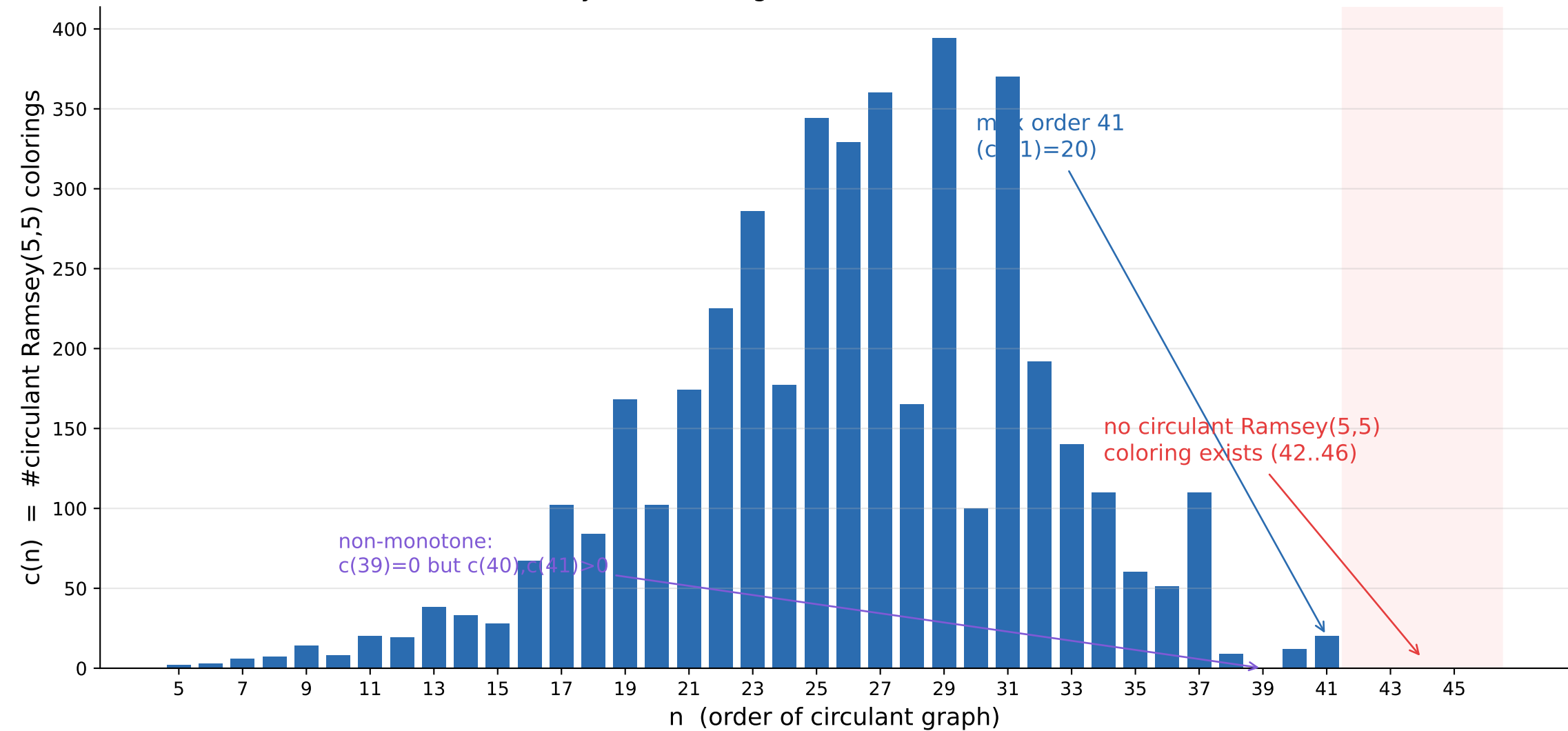
Circulant Ramsey(5,5) colorings: c(41)=20 max, c(n)=0 for 42 \leq n \leq 46
