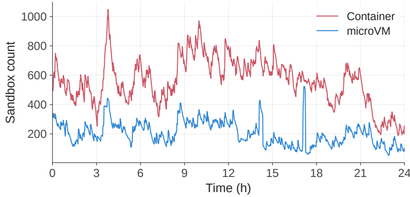
Figure 6 | The number of live sandboxes on one production node over a day. The observed peaks are 1,048 containers and 524 microVMs. Data were sampled over one day in early 2026.
