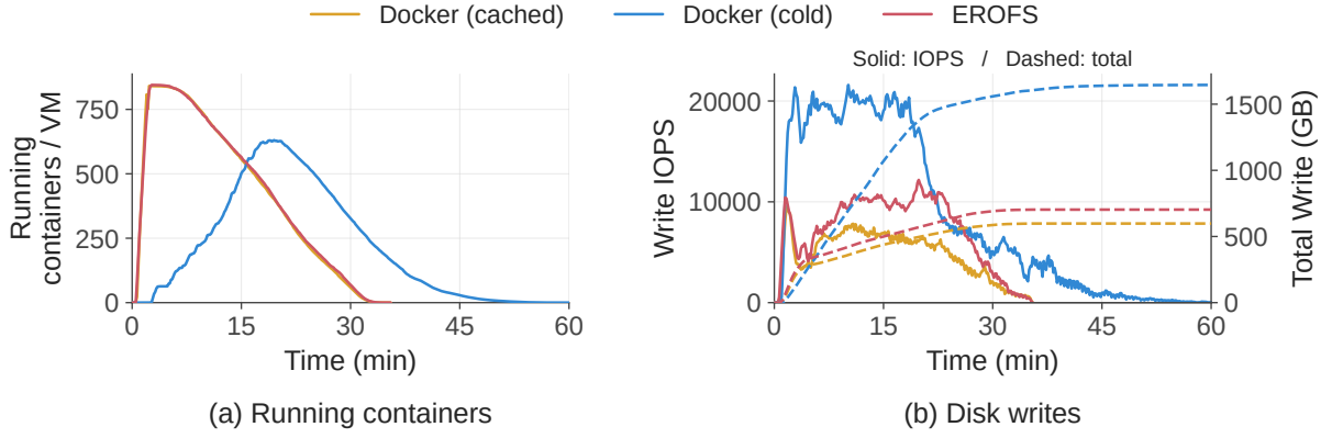
Figure 10 | On-demand EROFS pulling vs. eager Docker pulling (cold) and fully-local Docker (cached) under an 8,192-container burst across the 10-node evaluation cluster. Left: running-container count per node over time. Right: instantaneous disk-write IOPS (solid, left axis) and cumulative disk writes (dashed, right axis).
