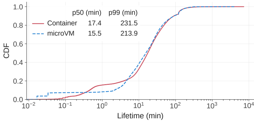
Figure 7 | Sandbox lifetime distributions sampled from 30K containers and 10K microVMs. Median lifetimes are 17.4 and 15.5 minutes, respectively, and p99 lifetimes exceed three hours for both backends. Data were sampled over one week in early 2026.
