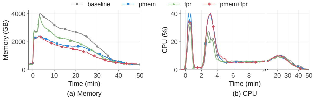
Figure 12 | Host memory usage (left) and CPU utilization (right) across the four Firecracker configurations under a real agentic RL workload. The CPU panel uses an expanded time scale for the first 10 minutes and a compressed scale for the 10–50 minute interval.
