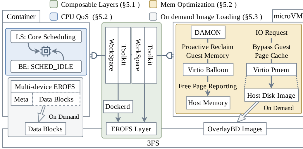
Figure 9 | Overview of the core system mechanisms. LS denotes latency-sensitive and BE denotes best-effort.
