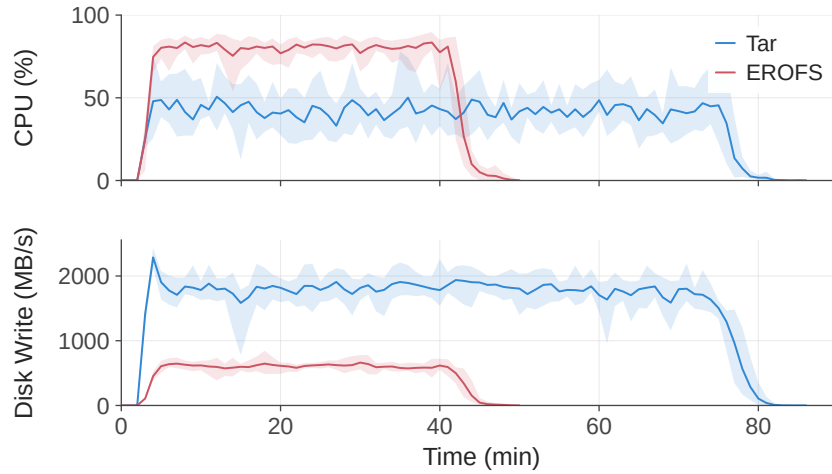
Figure 11 | Setup-phase CPU utilization and disk-write throughput when provisioning the evaluation workspace with per-sandbox tar extraction versus EROFS layer mounting.
