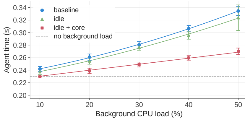
Figure 13 | Latency-sensitive agent time under increasing co-located best-effort CPU load, comparing an unprotected baseline, SCHED_IDLE alone, and SCHED_IDLE combined with core scheduling.
