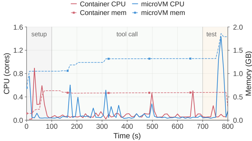
Figure 3 | A representative sandbox execution with setup, tool-call, and test phases. CPU demand is intermittent after setup, while the memory footprint and accumulated state persist.
