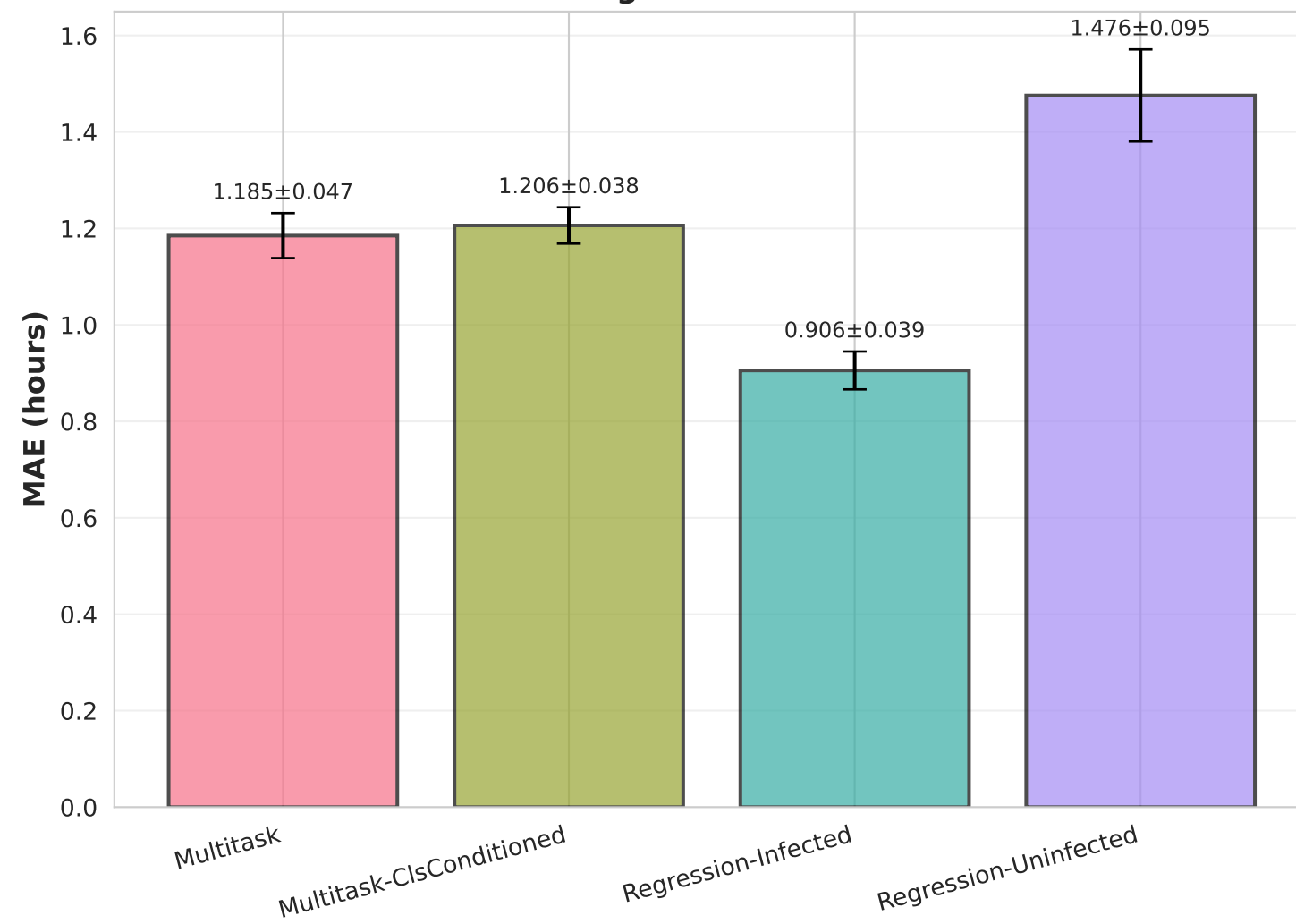
Regression MAE
