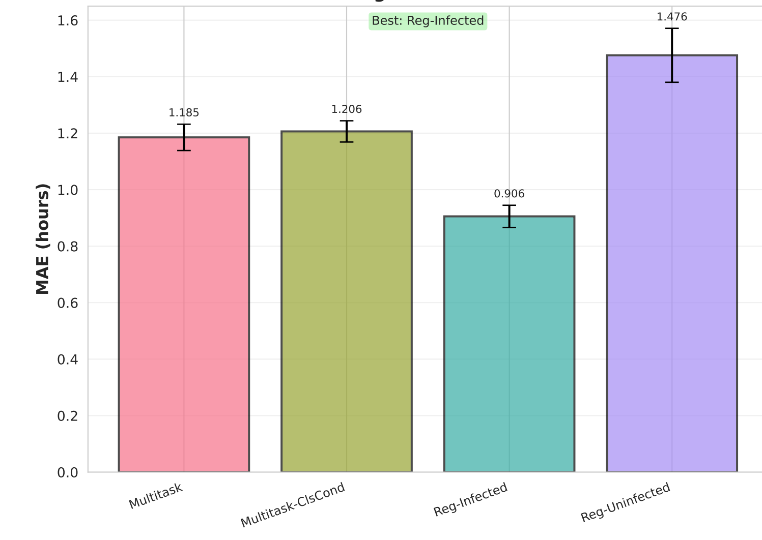
Regression MAE
