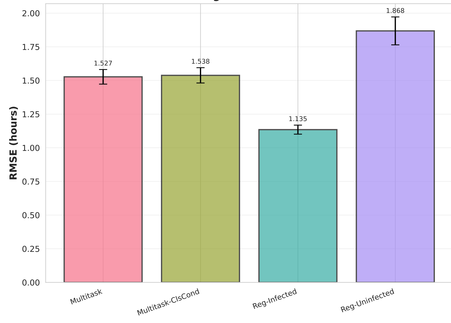
Regression RMSE
