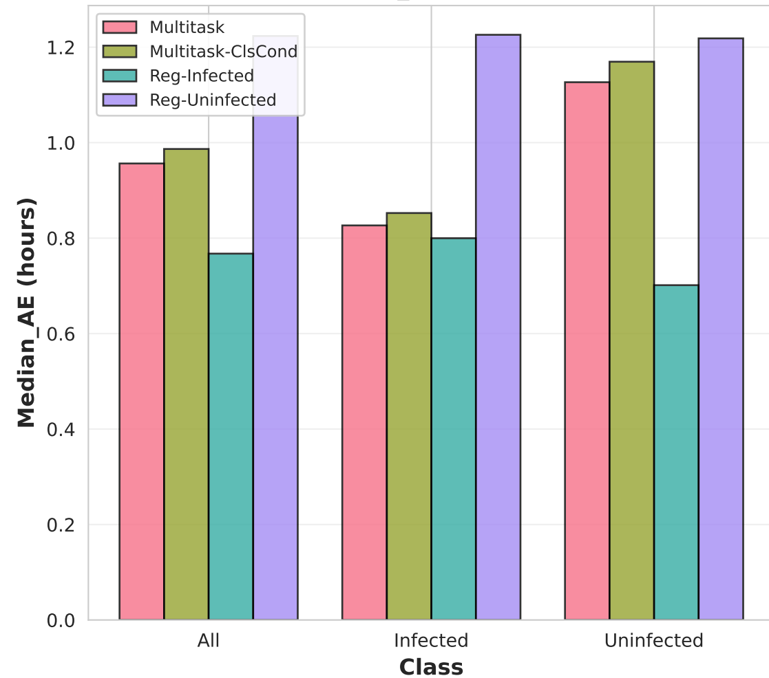
Median_AE by Class
