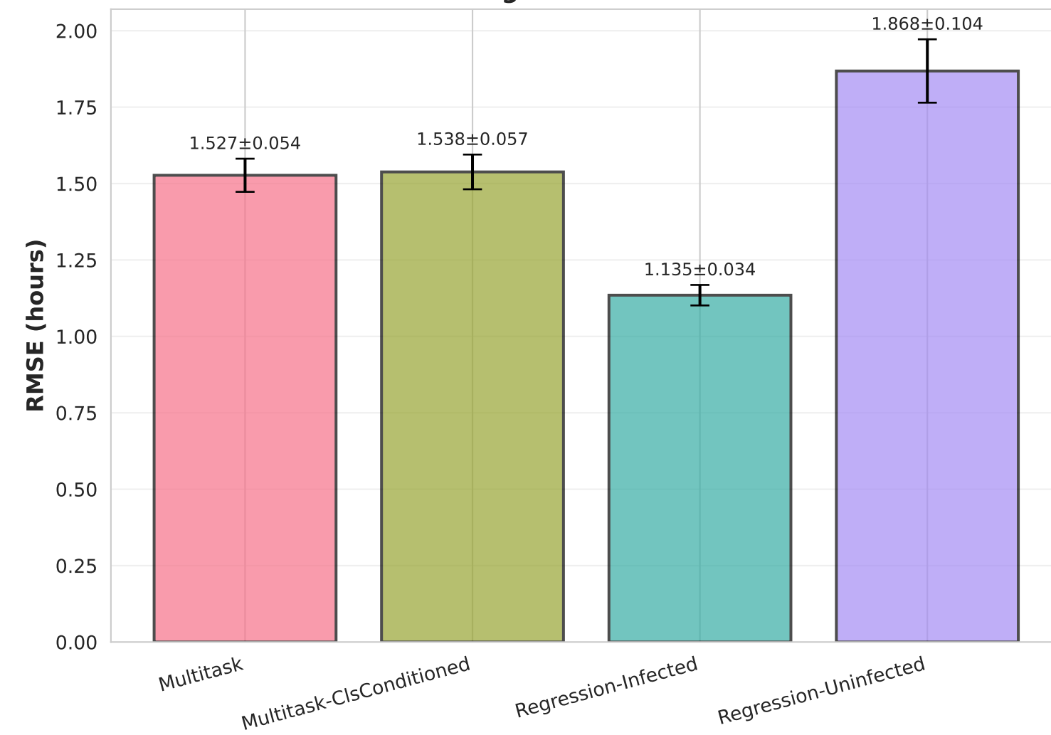
Regression RMSE
