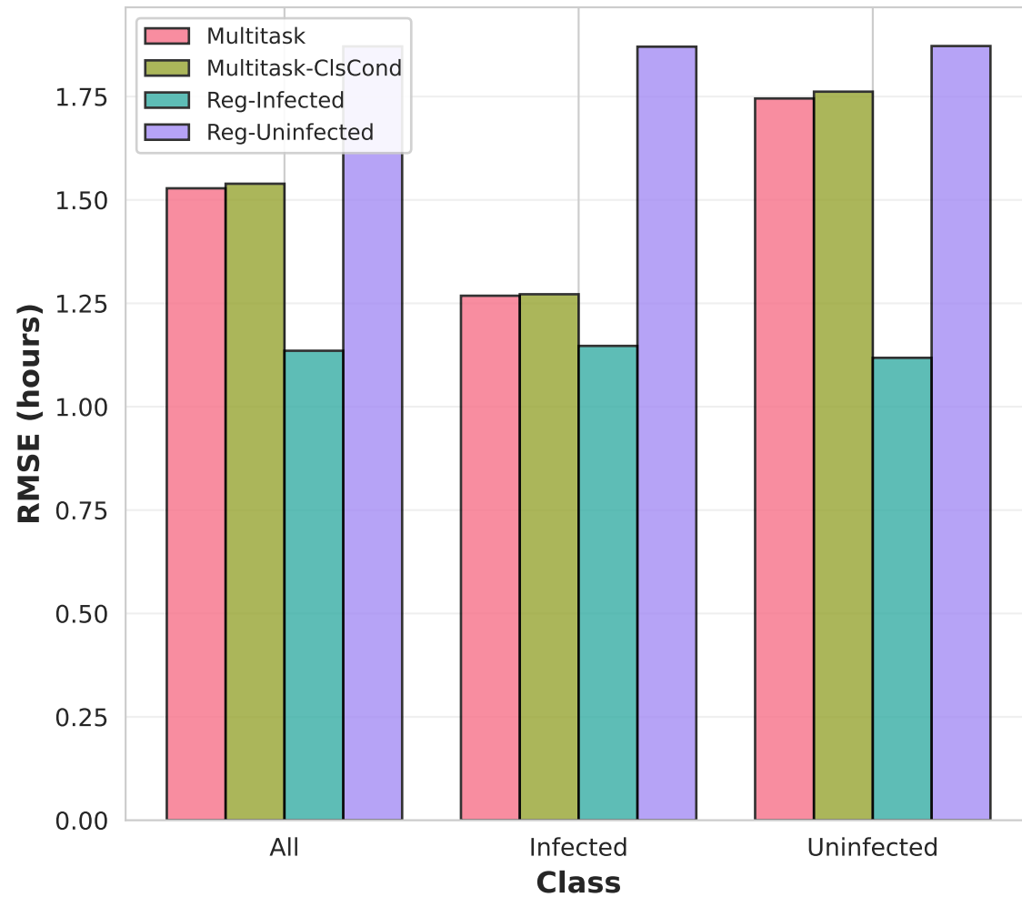
RMSE by Class
