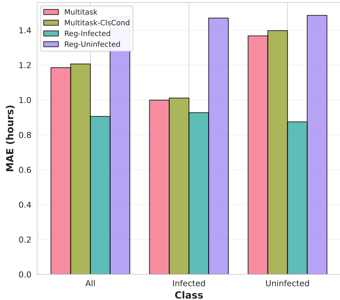
MAE by Class
