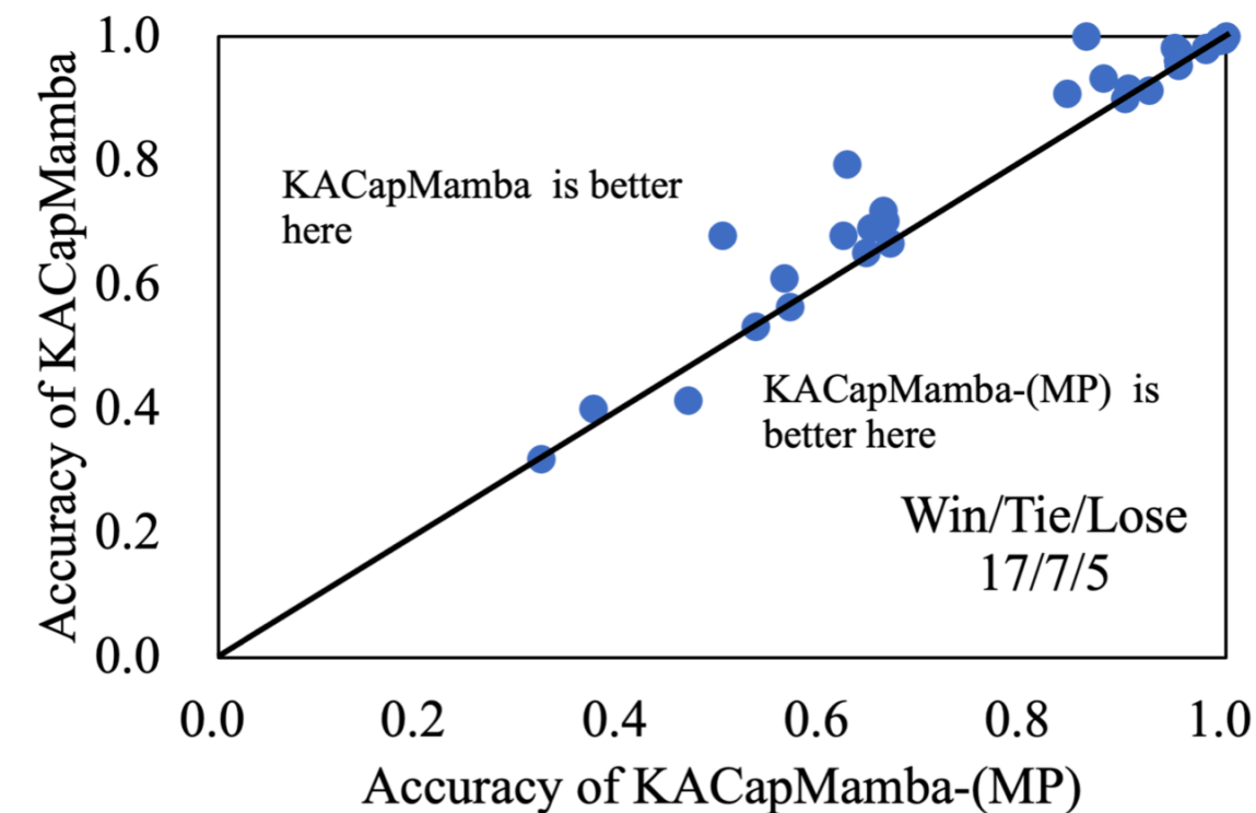
(e) KACapMamba-(MP) vs. KACapMamba
