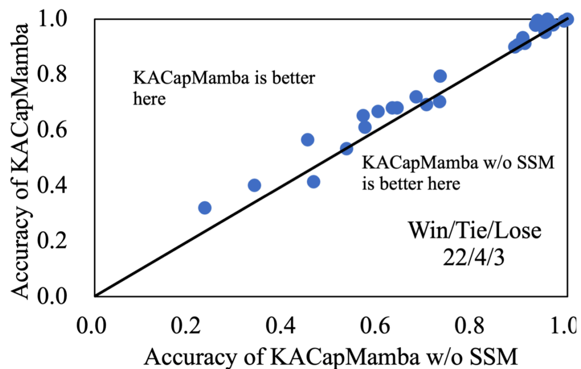
(b) KACapMamba w/o SSM vs. KACapMamba
