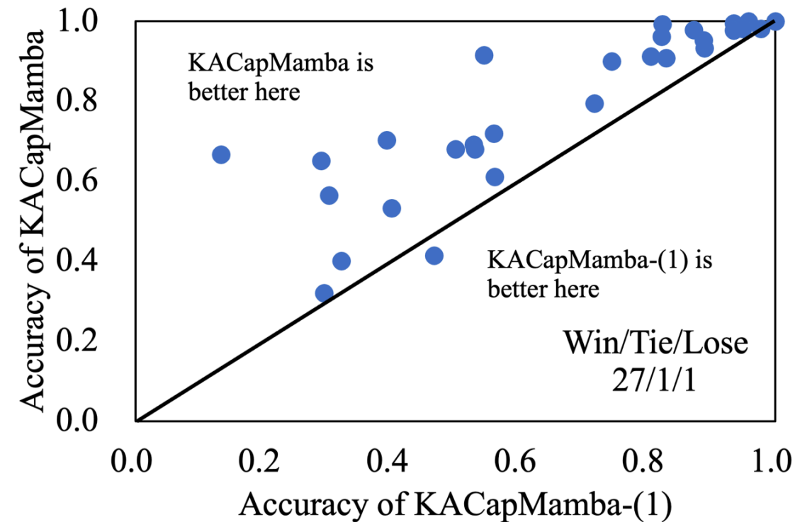
(a) KACapMamba-1 vs. KACapMamba
