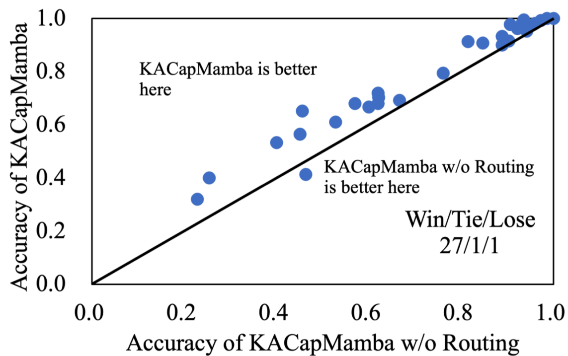
(a) KACapMamba w/o Routing vs. KACapMamba
