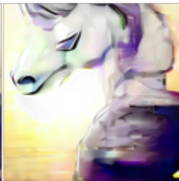
TaylorSeer mech.
