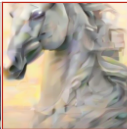
trajectory objective
